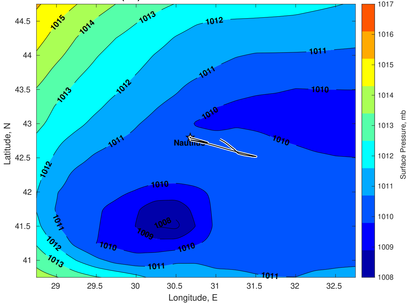
Surface Pressure (mb) for Nautilus at 08-Dec-2025 00:00:00
