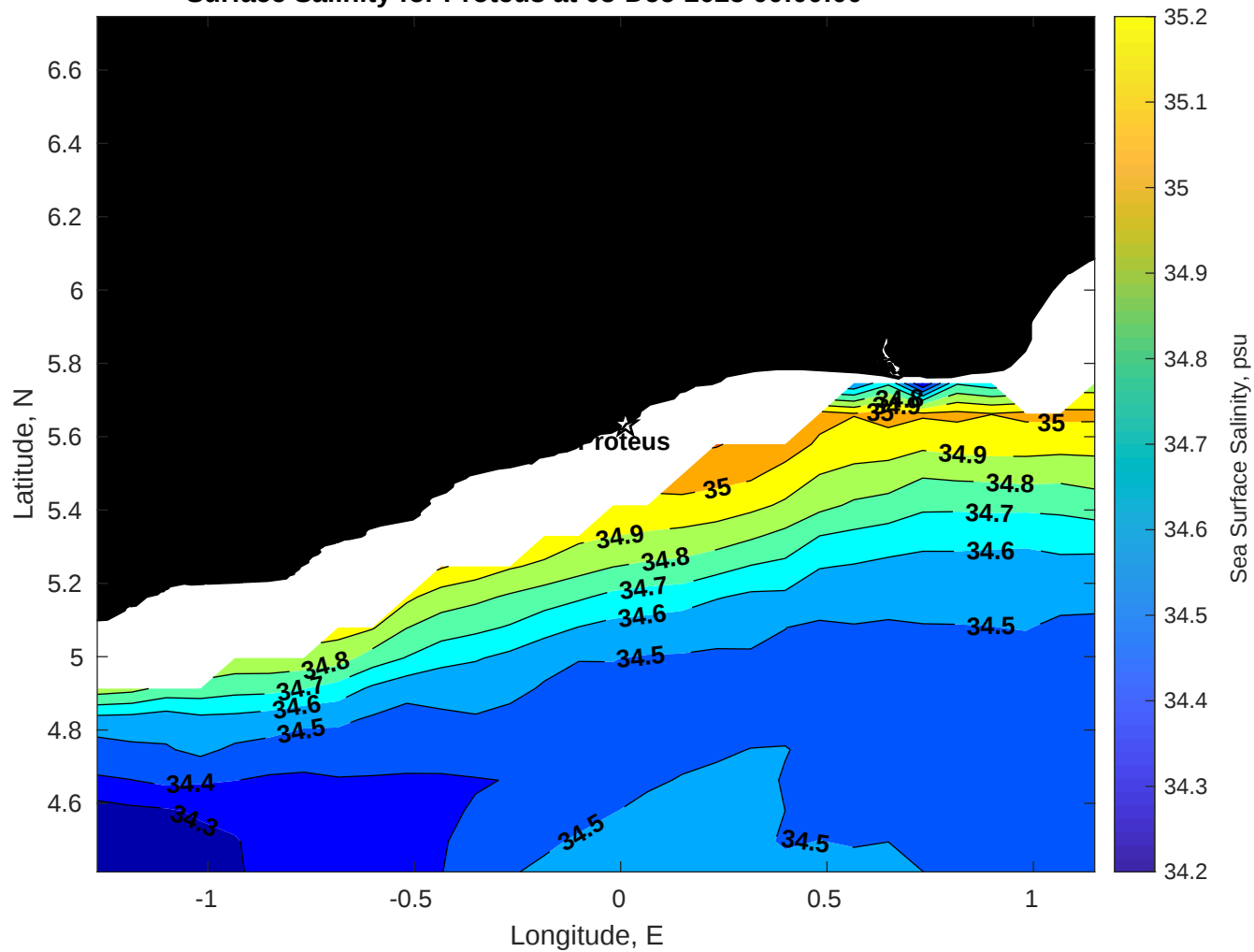
Surface Salinity for Proteus at 05-Dec-2025 00:00:00
