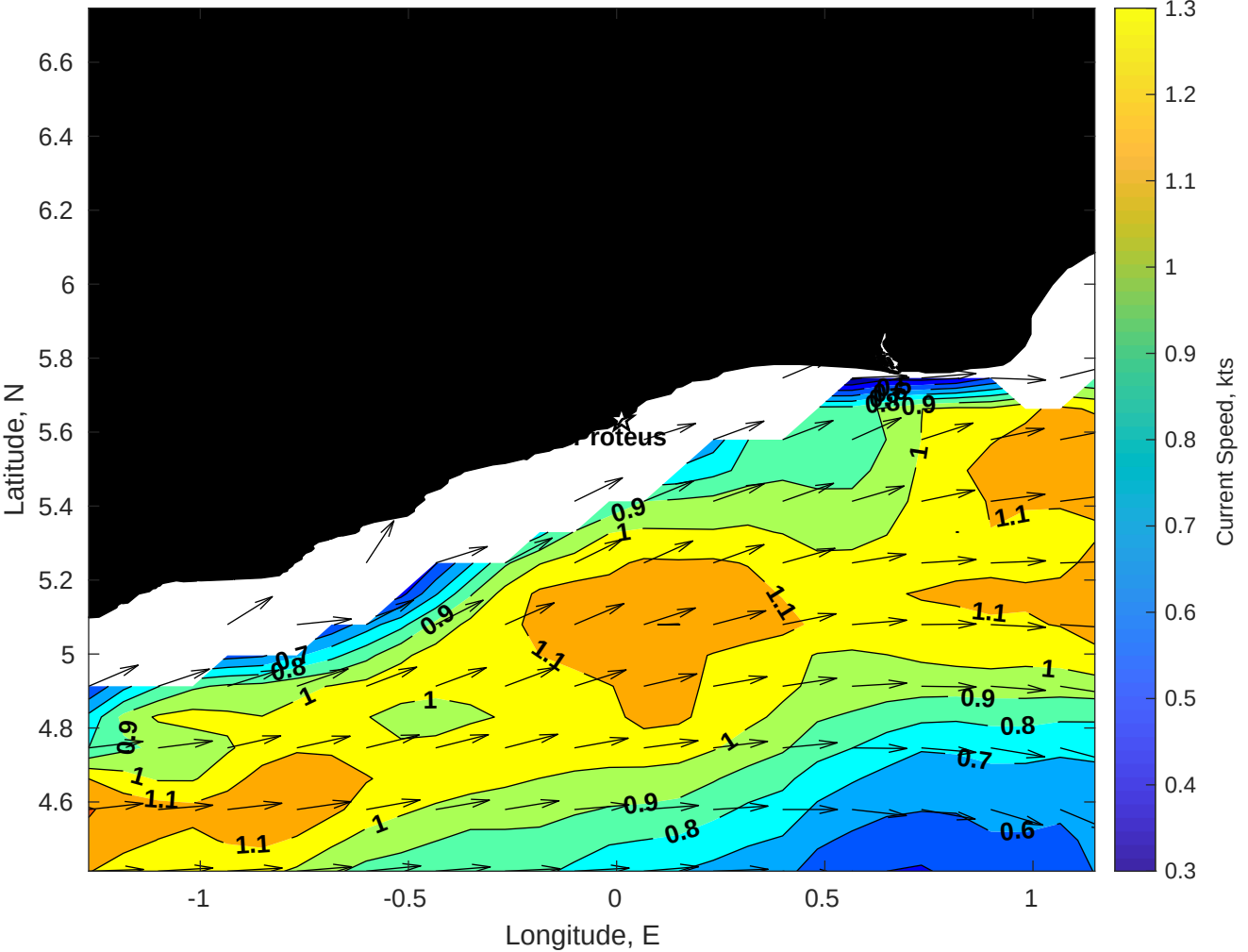
Surface Currents for Proteus at 05-Dec-2025 00:00:00
