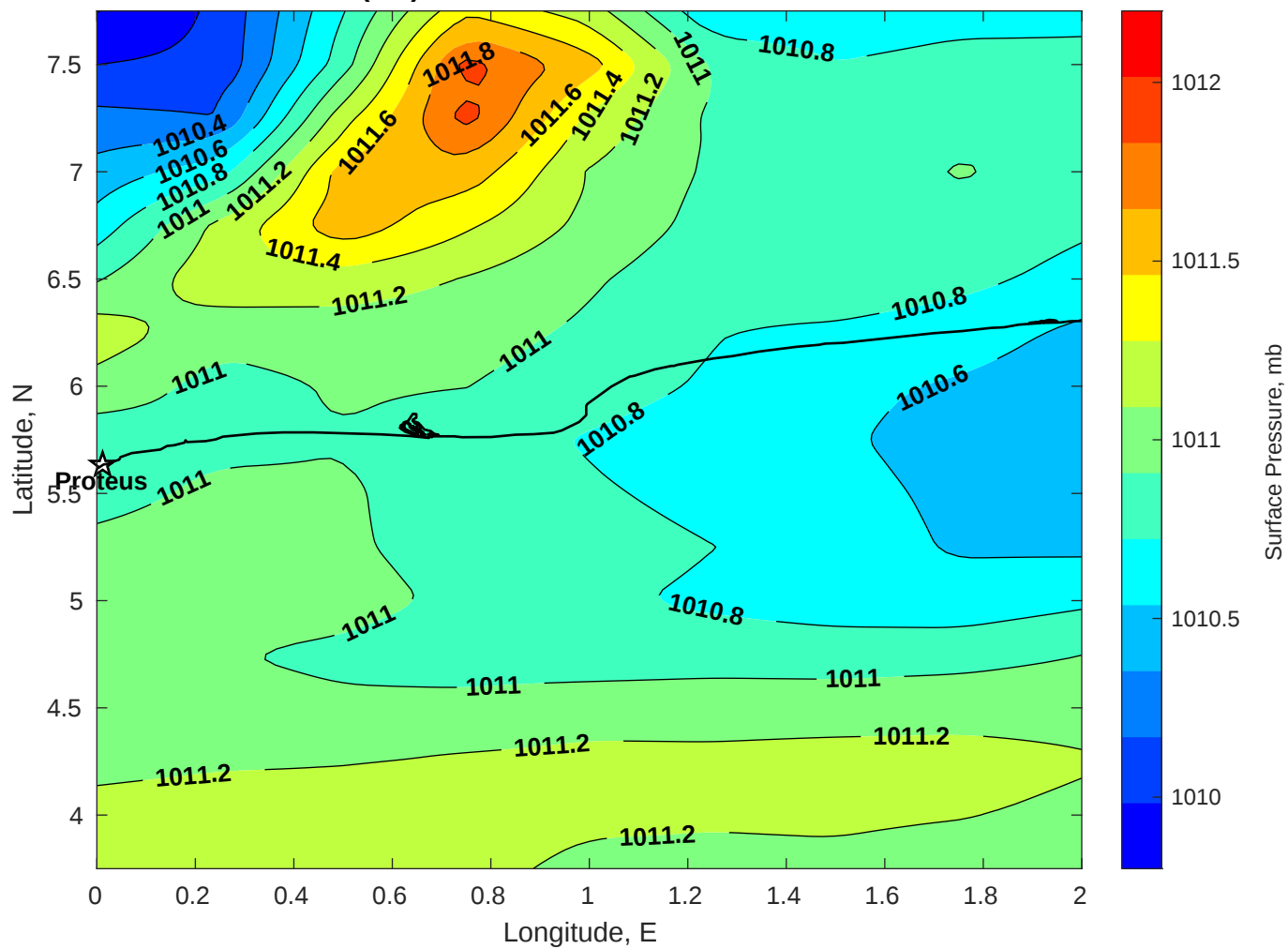
Surface Pressure (mb) for Proteus at 06-Dec-2025 00:00:00
