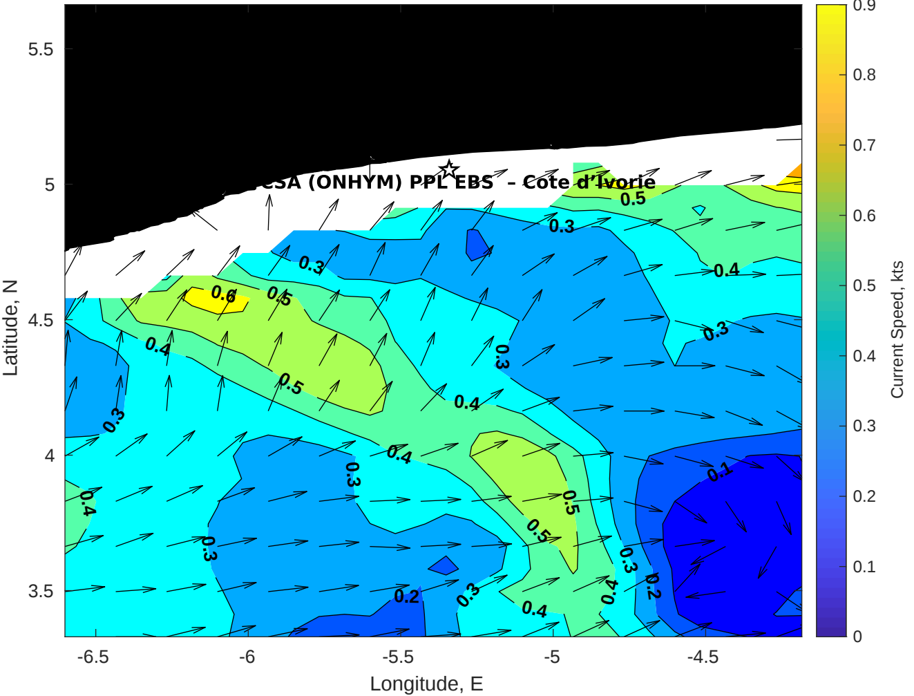
Surface Currents for CSA (ONHYM) PPL EBS - Cote d'Ivoire at 06-Dec-2025 00:00:00
