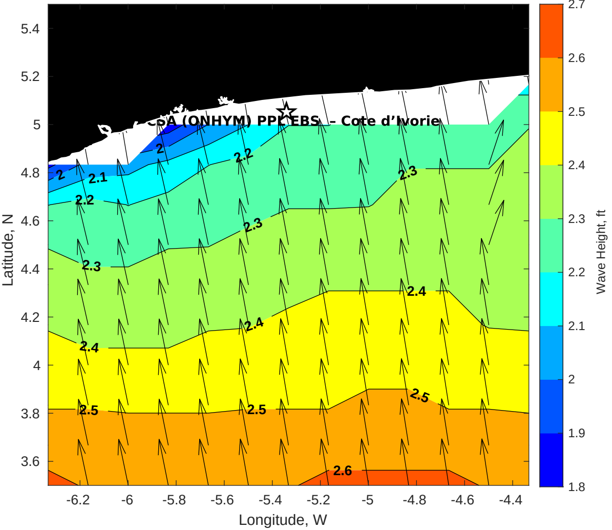
GFS Wave Height (ft) for CSA (ONHYM) PPL EBS - Cote d'Ivoire at 07-Dec-2025 09:00:00
