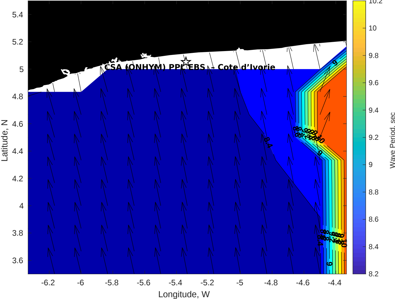
GFS Wave Period (sec) for CSA (ONHYM) PPL EBS - Cote d'Ivoire at 07-Dec-2025 09:00:00
