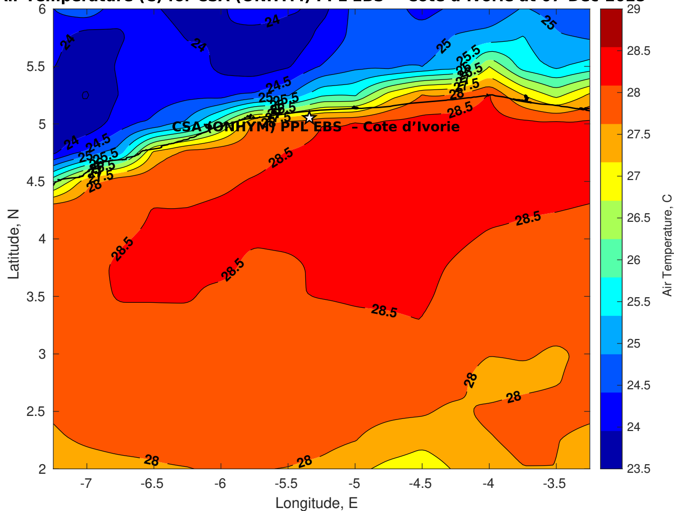
Air Temperature (C) for CSA (ONHYM) PPL EBS - Cote d'Ivoire at 07-Dec-2025
