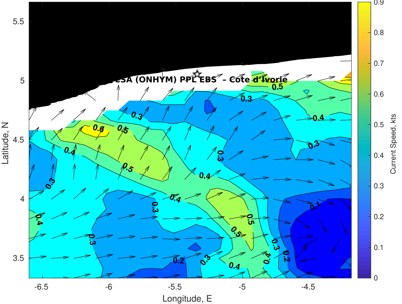
Surface Currents for CSA (ONHYM) PPL EBS - Cote d'Ivoire at 06-Dec-2025 00:00:00
