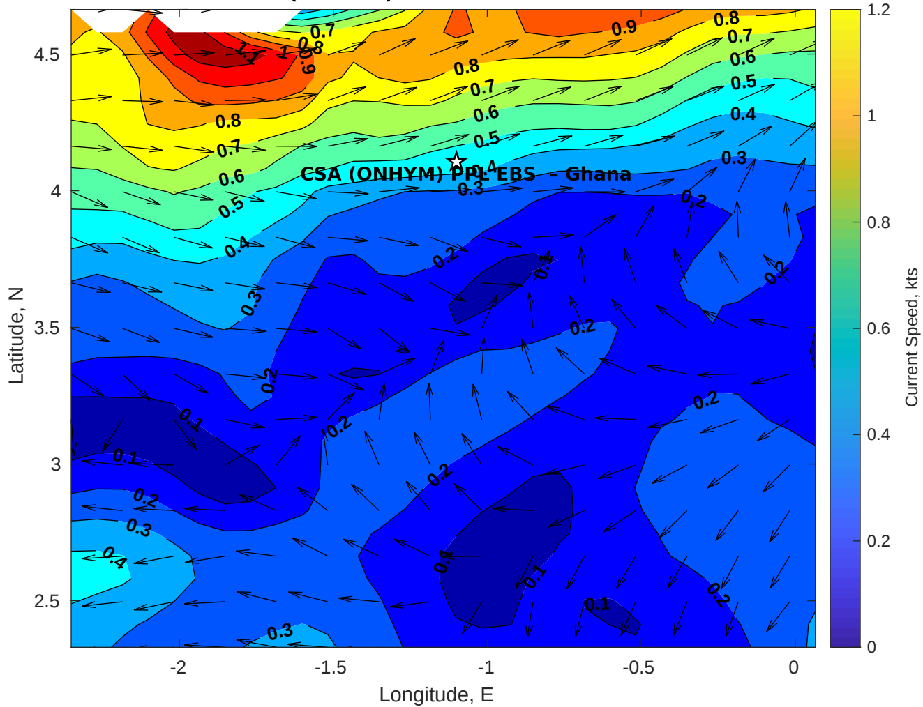
Surface Currents for CSA (ONHYM) PPL EBS - Ghana at 06-Dec-2025 00:00:00
