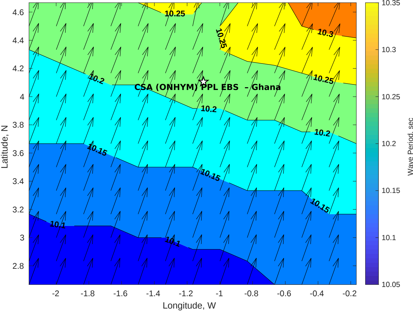
GFS Wave Period (sec) for CSA (ONHYM) PPL EBS - Ghana at 07-Dec-2025 09:00:00
