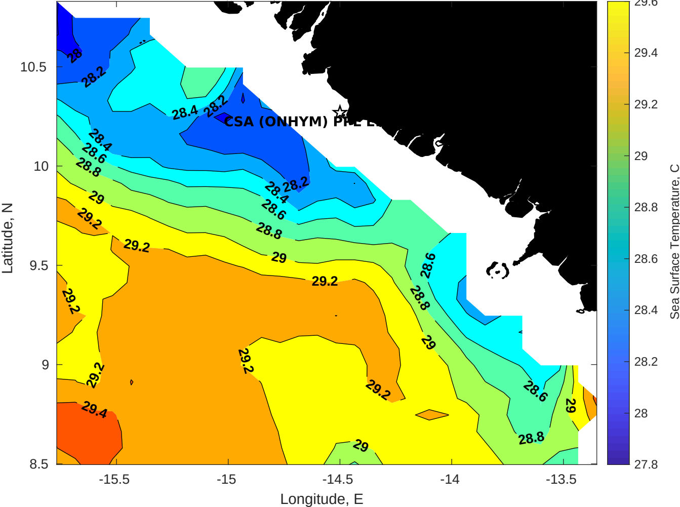
SST for CSA (ONHYM) PPL EBS - Guinea at 06-Dec-2025 00:00:00
