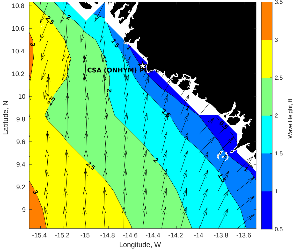
GFS Wave Height (ft) for CSA (ONHYM) PPL EBS - Guinea at 07-Dec-2025 09:00:00
