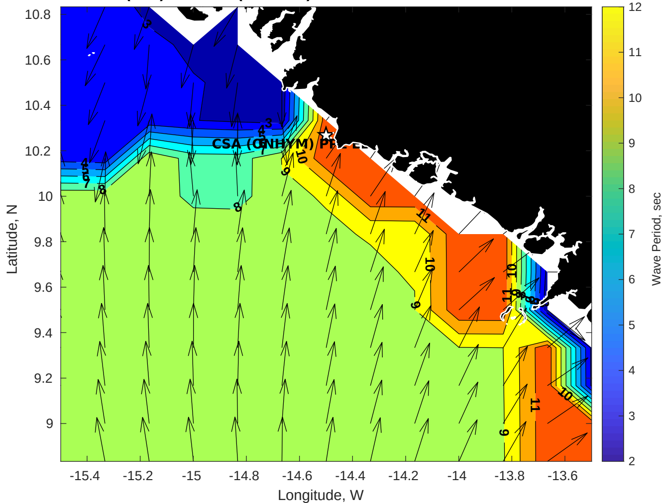
GFS Wave Period (sec) for CSA (ONHYM) PPL EBS - Guinea at 07-Dec-2025 09:00:00
