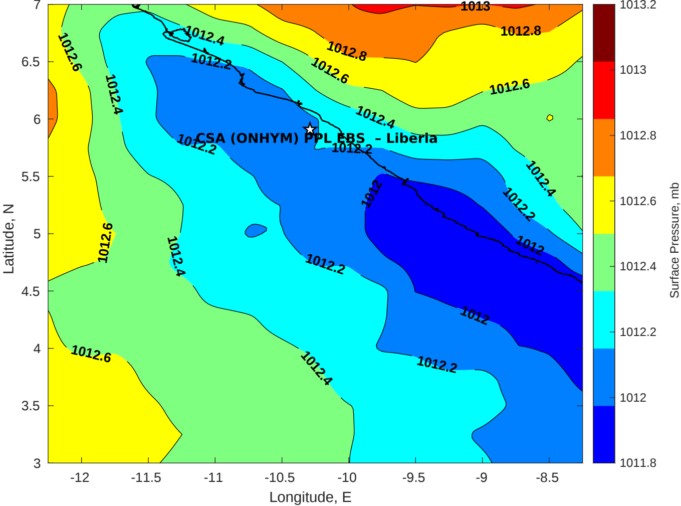
Surface Pressure (mb) for CSA (ONHYM) PPL EBS - Liberia at 07-Dec-2025 00:00:00
