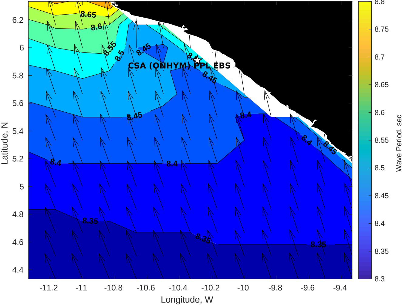
GFS Wave Period (sec) for CSA (ONHYM) PPL EBS - Liberia at 07-Dec-2025 09:00:00
