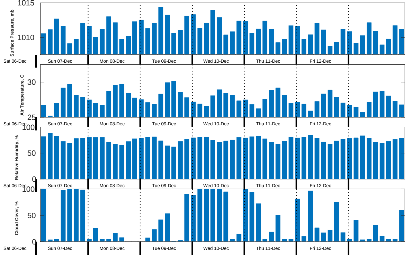
Met Forecast for CSA (ONHYM) PPL EBS - Liberia from 07-Dec-2025 00:00:00 to 14-Dec-2025 00:00:00
