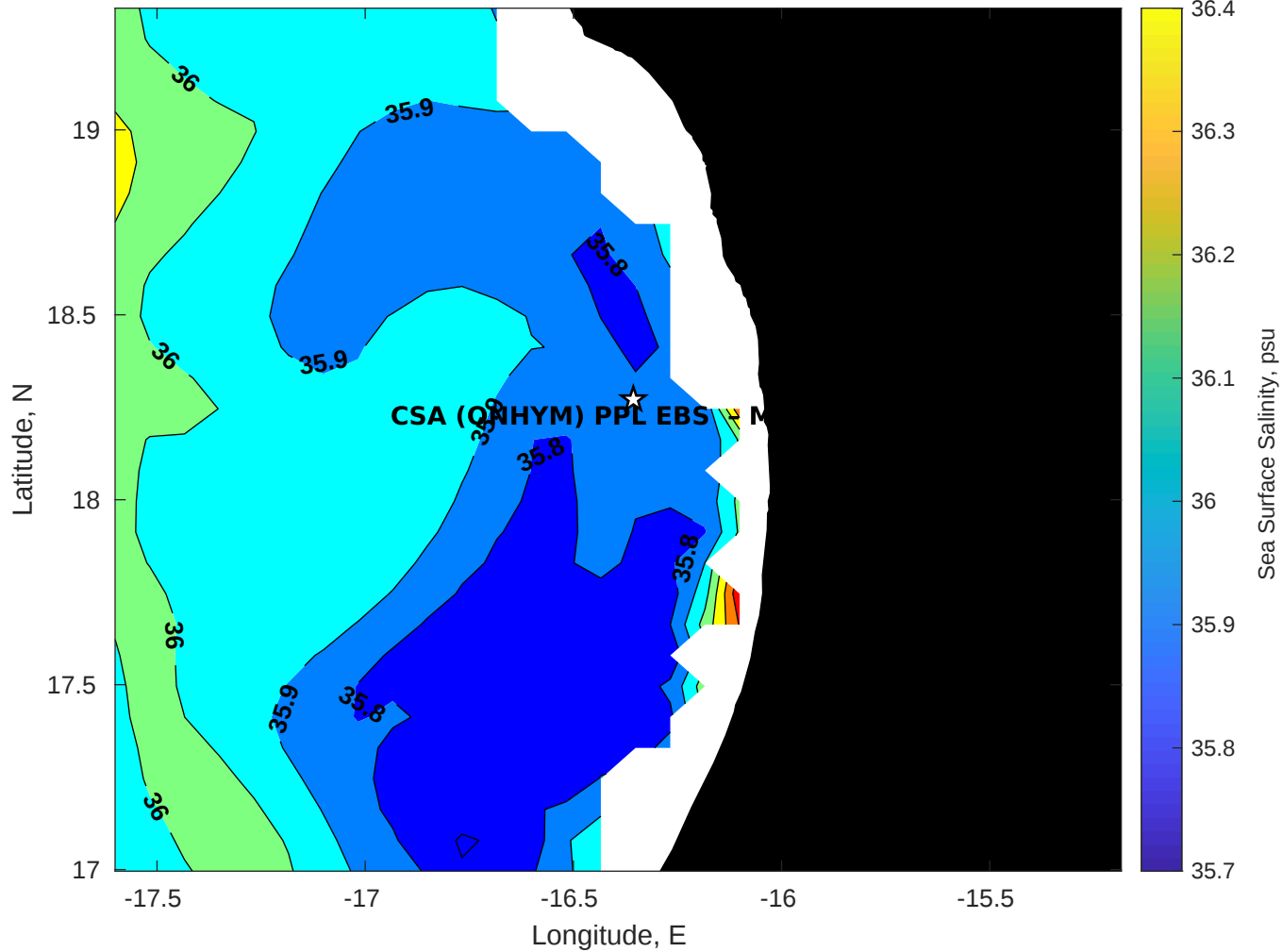
Surface Salinity for CSA (ONHYM) PPL EBS - Mauritania at 06-Dec-2025 00:00:00
