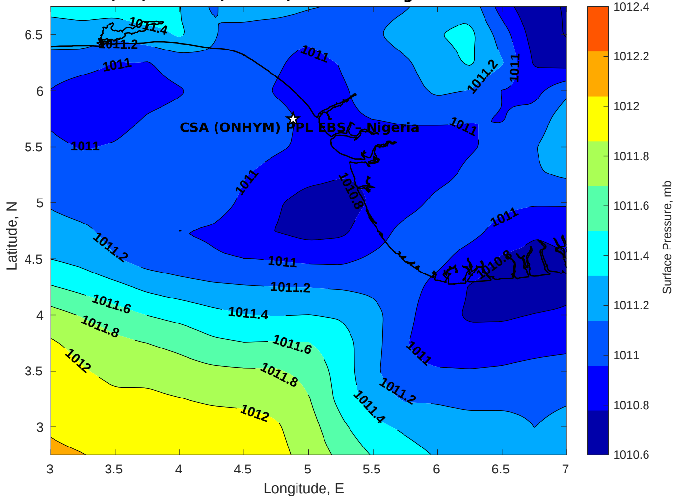
Surface Pressure (mb) for CSA (ONHYM) PPL EBS - Nigeria at 09-Dec-2025 00:00:00
