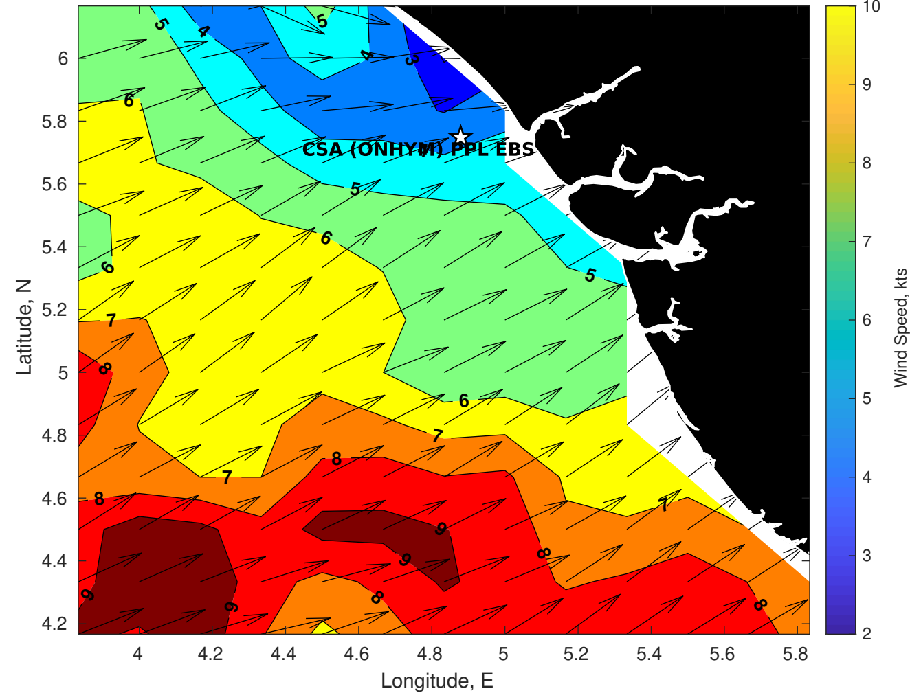
GFS Winds (kts) for CSA (ONHYM) PPL EBS - Nigeria at 07-Dec-2025 09:00:00
