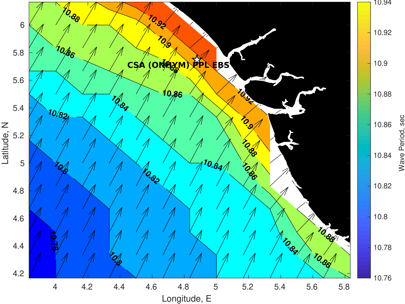
GFS Wave Period (sec) for CSA (ONHYM) PPL EBS - Nigeria at 07-Dec-2025 09:00:00
