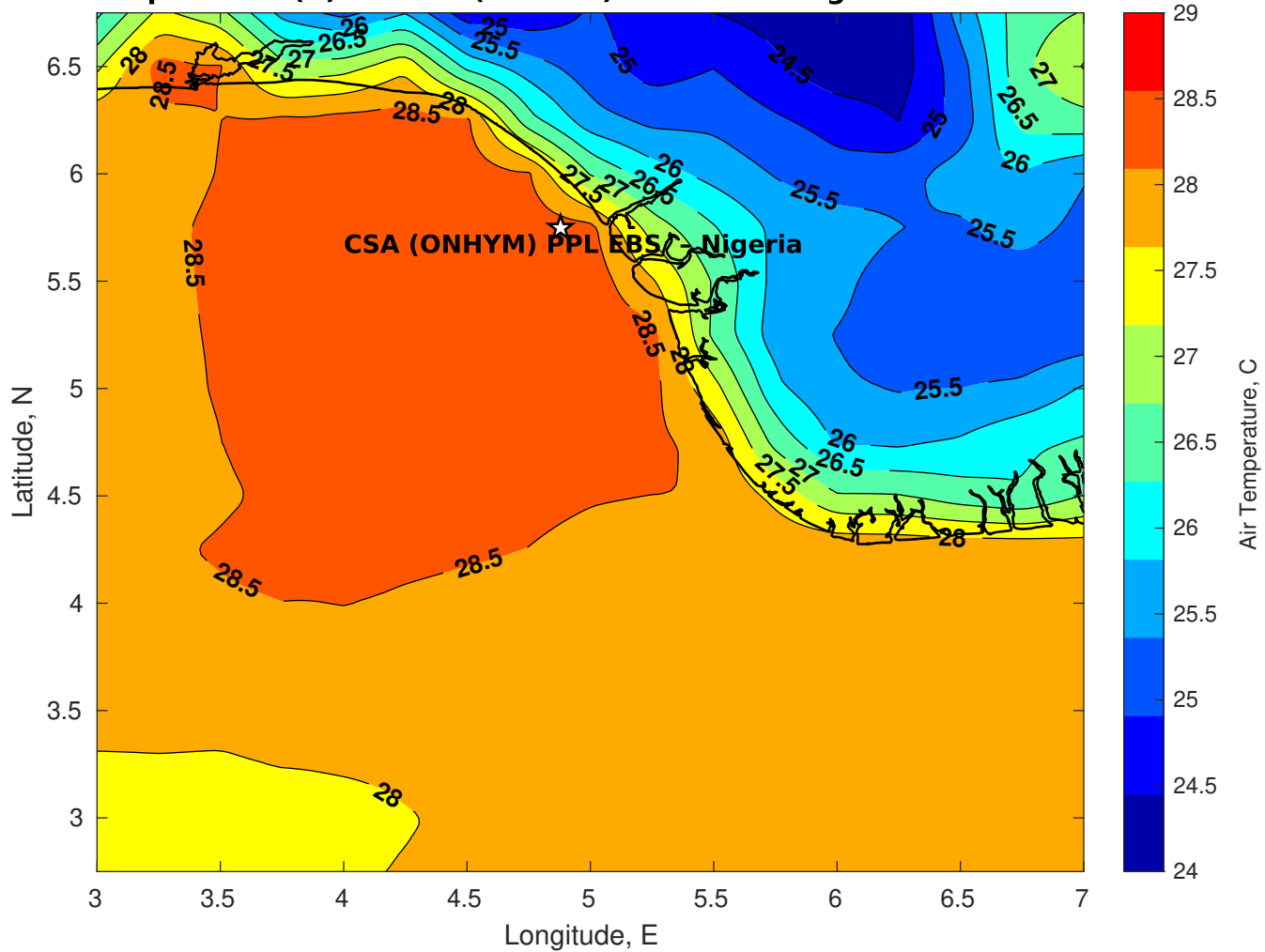
Air Temperature (C) for CSA (ONHYM) PPL EBS - Nigeria at 07-Dec-2025
