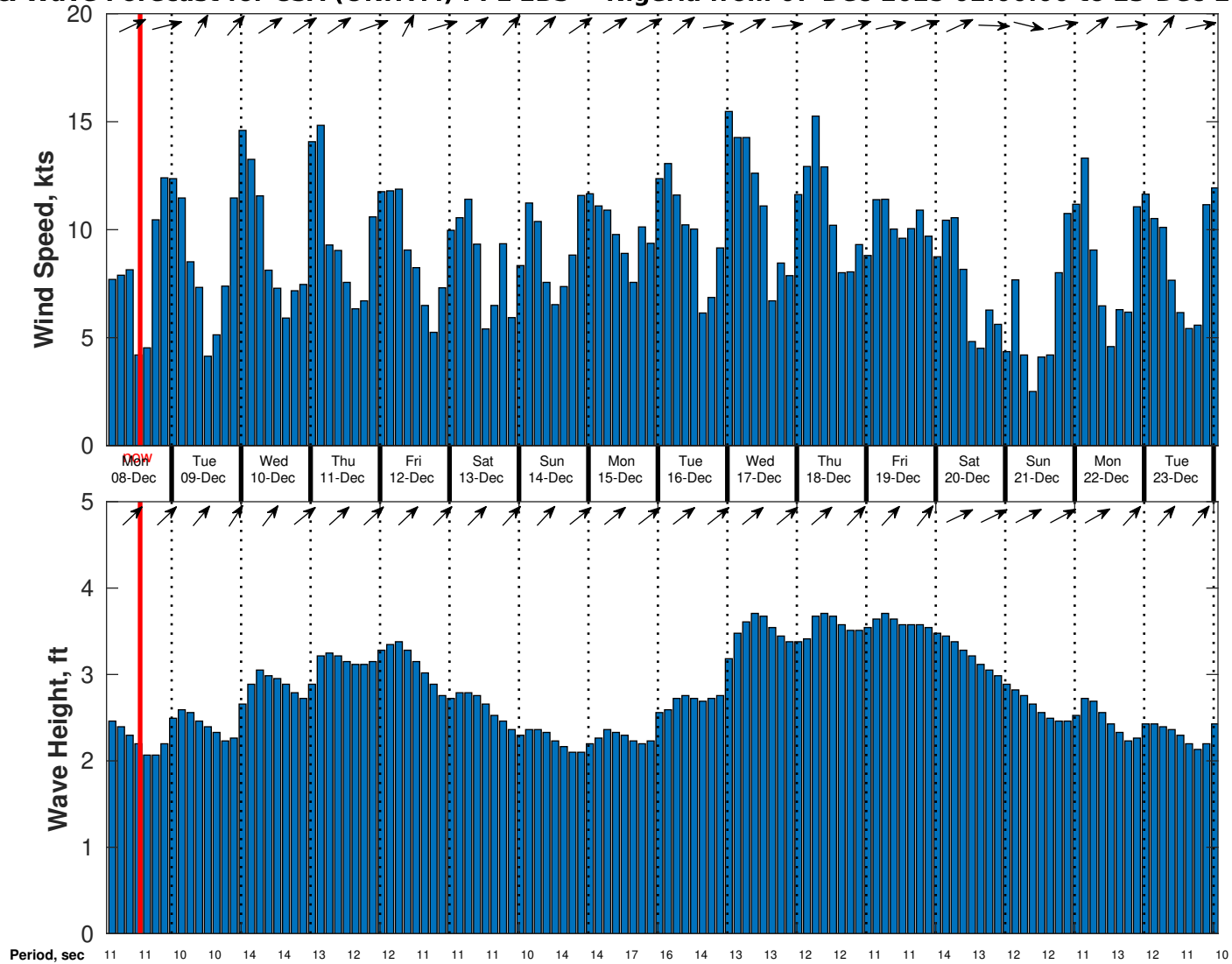
Wind & Wave Forecast for CSA (ONHYM) PPL EBS - Nigeria from 07-Dec-2025 02:00:00 to 23-Dec-2025 02:00:00
