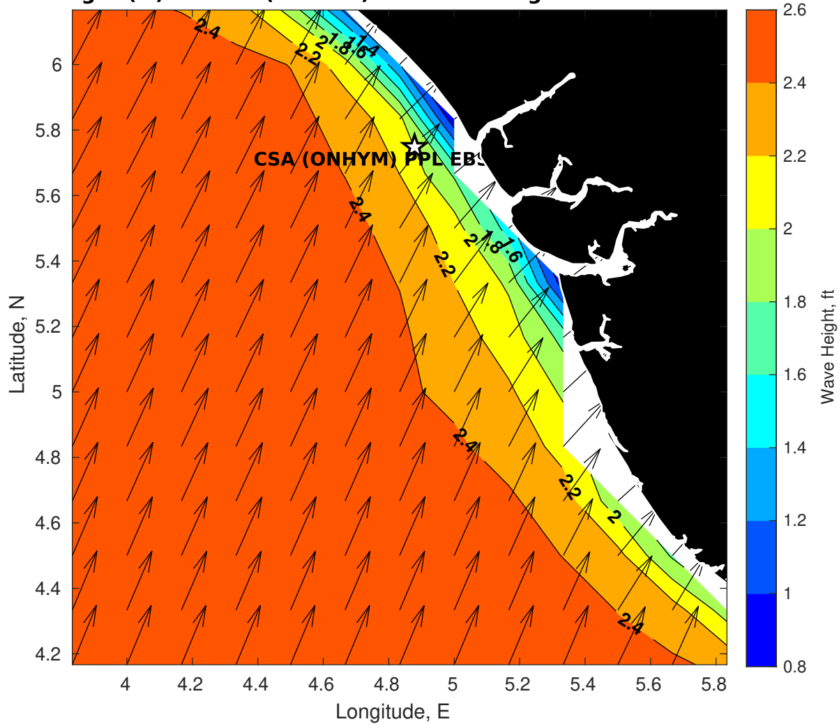
GFS Wave Height (ft) for CSA (ONHYM) PPL EBS - Nigeria at 07-Dec-2025 09:00:00
