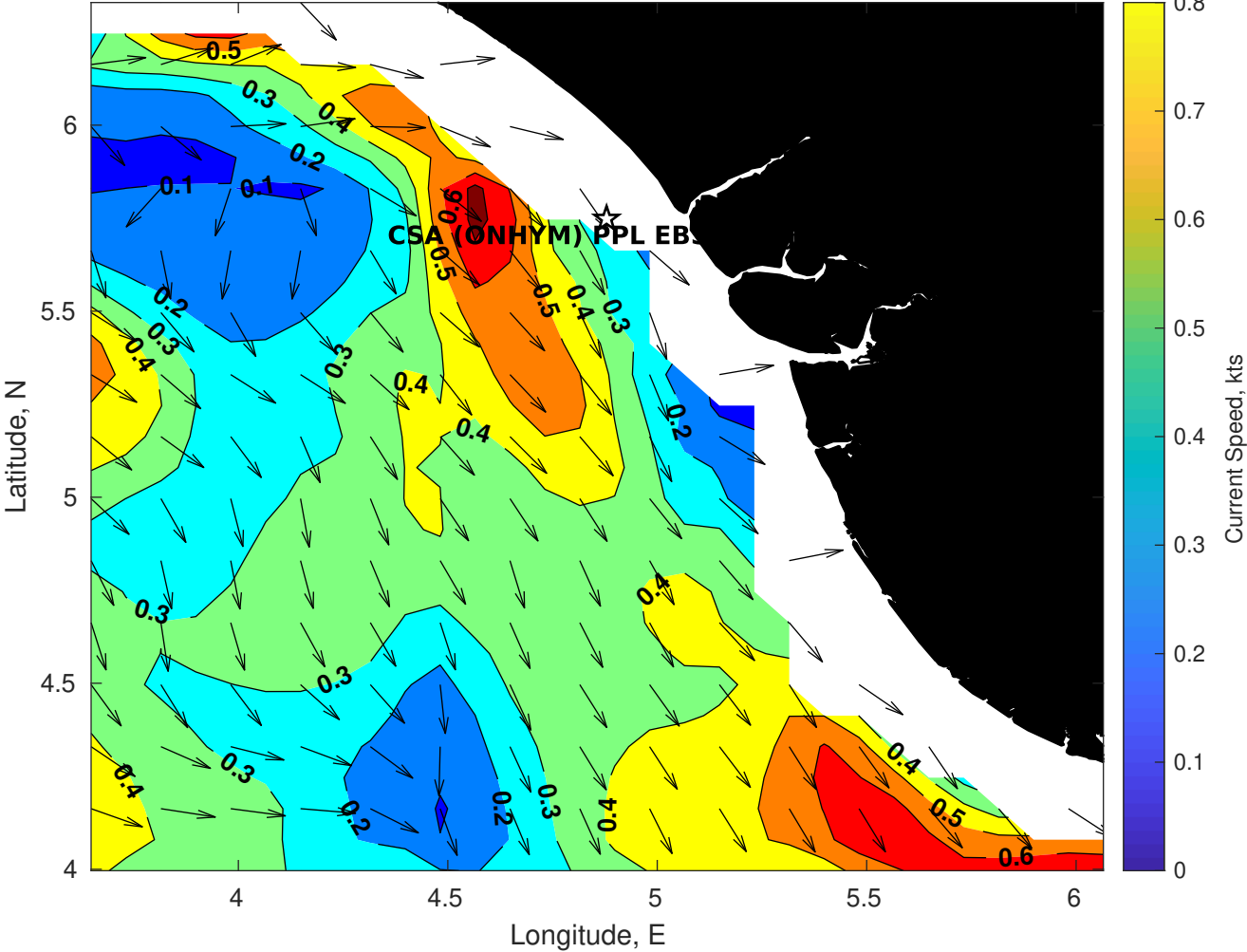
Surface Currents for CSA (ONHYM) PPL EBS - Nigeria at 06-Dec-2025 00:00:00
