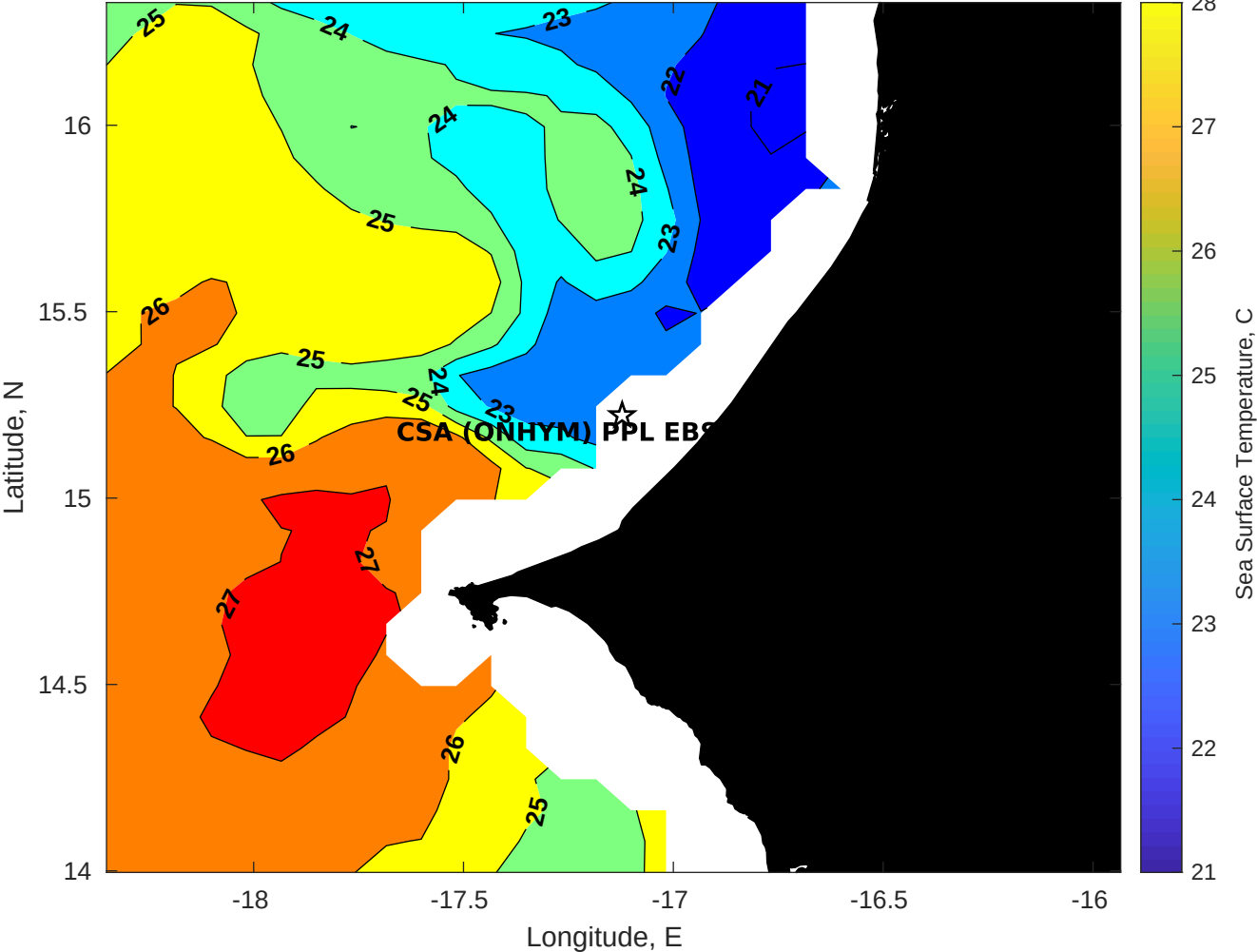
SST for CSA (ONHYM) PPL EBS - Senegal at 06-Dec-2025 00:00:00
