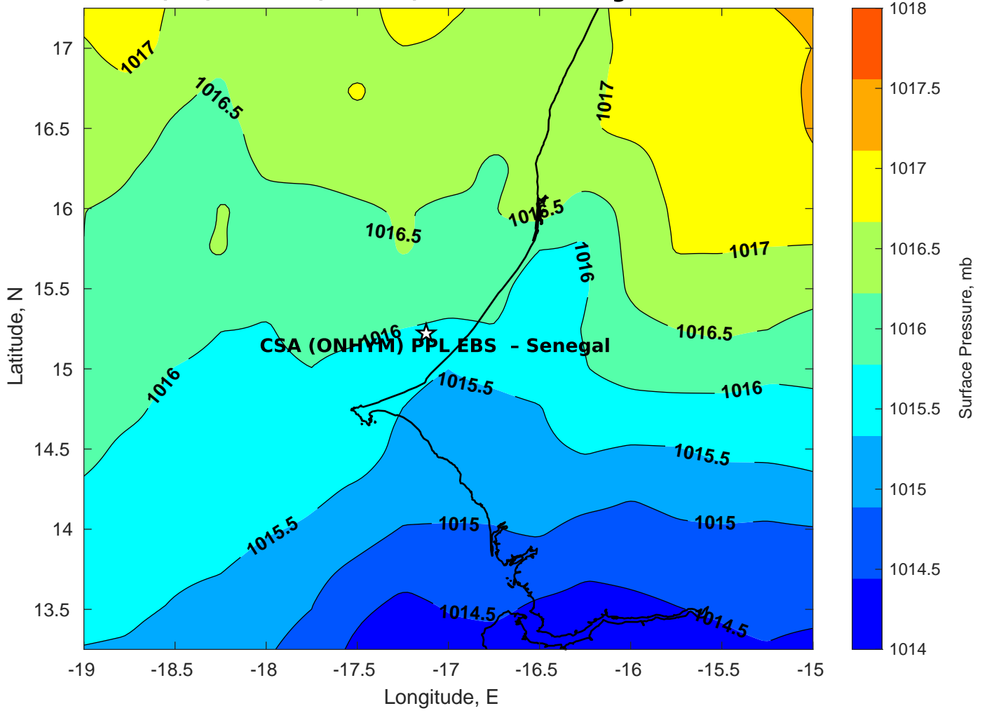
Surface Pressure (mb) for CSA (ONHYM) PPL EBS - Senegal at 07-Dec-2025 00:00:00
