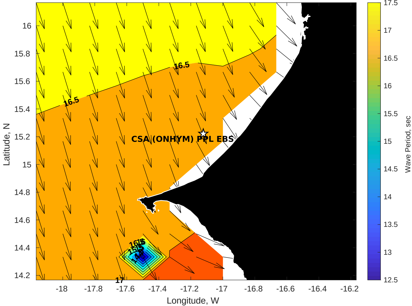
GFS Wave Period (sec) for CSA (ONHYM) PPL EBS - Senegal at 07-Dec-2025 09:00:00
