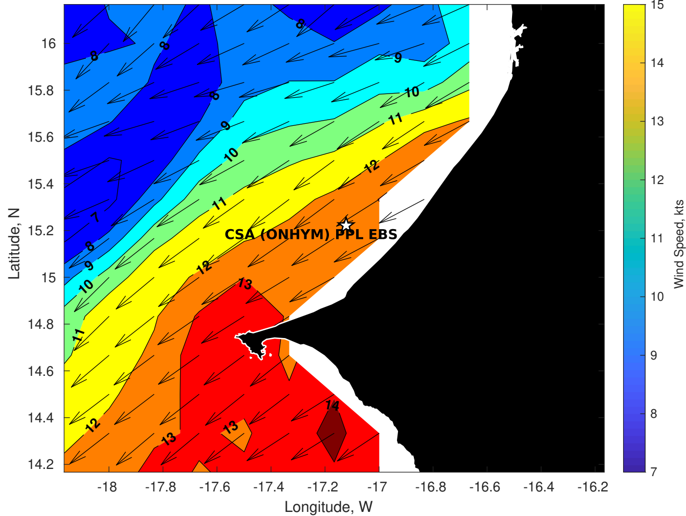
GFS Winds (kts) for CSA (ONHYM) PPL EBS - Senegal at 07-Dec-2025 09:00:00
