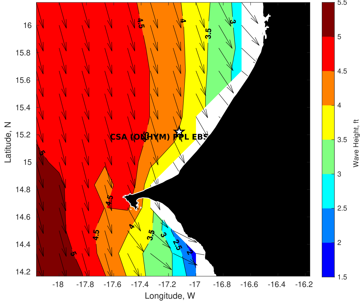
GFS Wave Height (ft) for CSA (ONHYM) PPL EBS - Senegal at 07-Dec-2025 09:00:00
