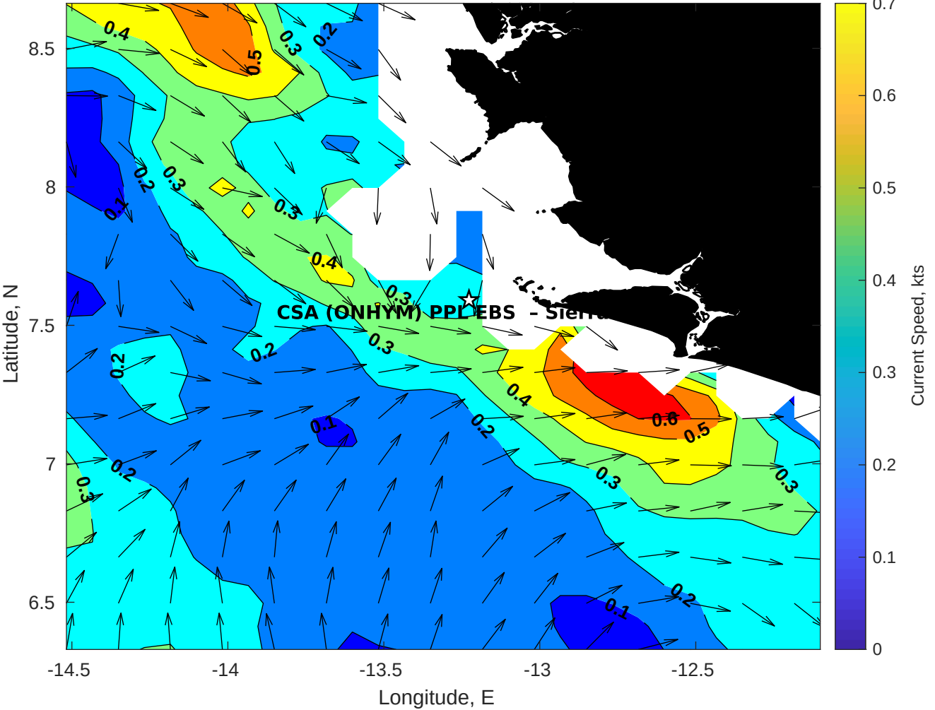
Surface Currents for CSA (ONHYM) PPL EBS - Sierra Leone at 06-Dec-2025 00:00:00
