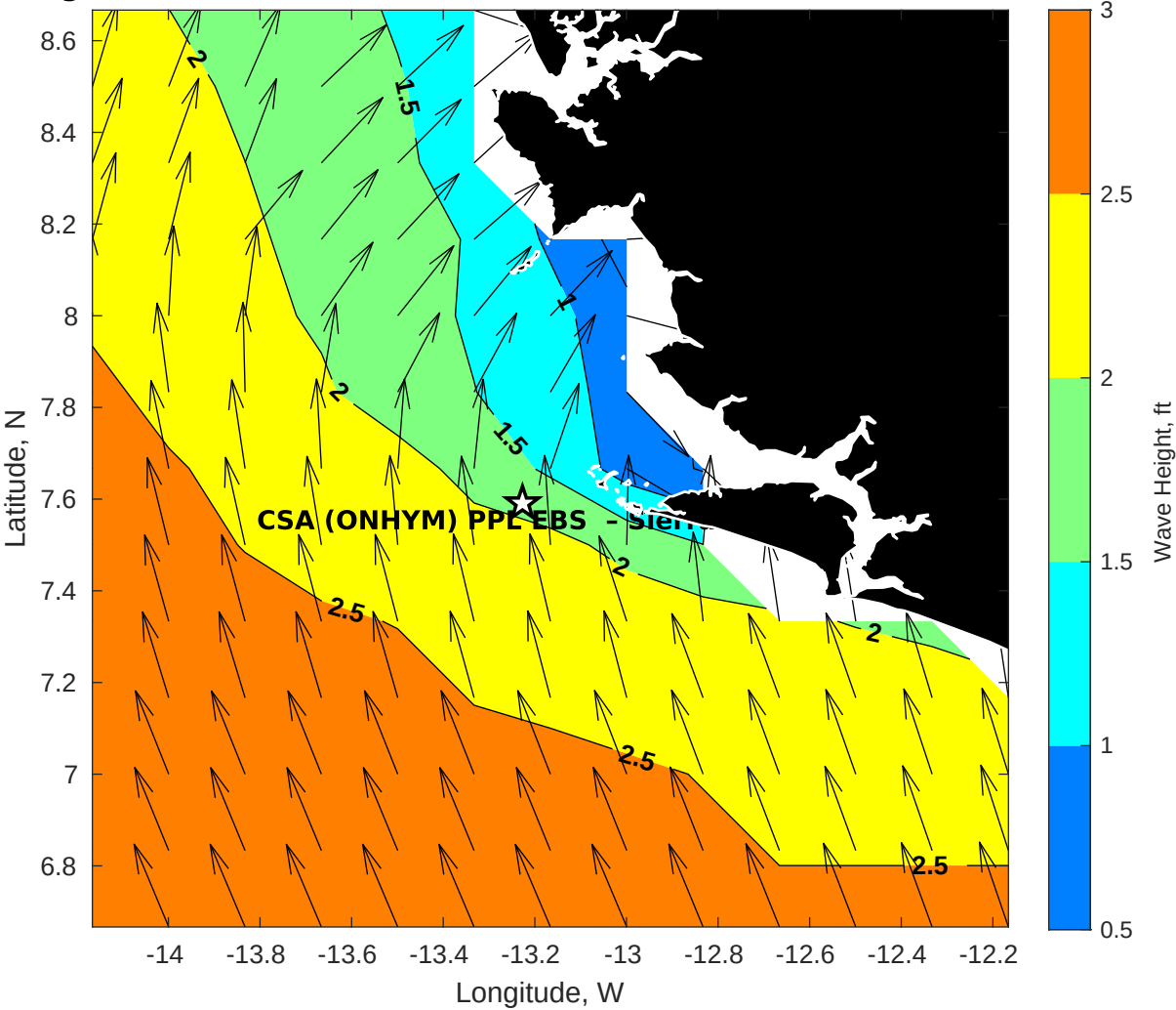
GFS Wave Height (ft) for CSA (ONHYM) PPL EBS - Sierra Leone at 07-Dec-2025 09:00:00
