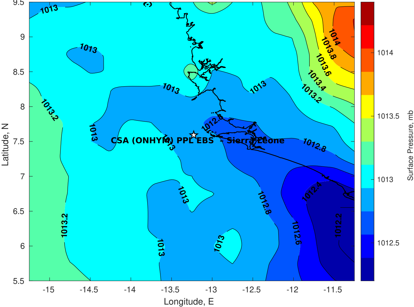
Surface Pressure (mb) for CSA (ONHYM) PPL EBS - Sierra Leone at 07-Dec-2025 00:00:00
