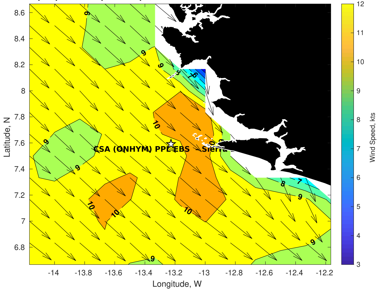
GFS Winds (kts) for CSA (ONHYM) PPL EBS - Sierra Leone at 07-Dec-2025 09:00:00
