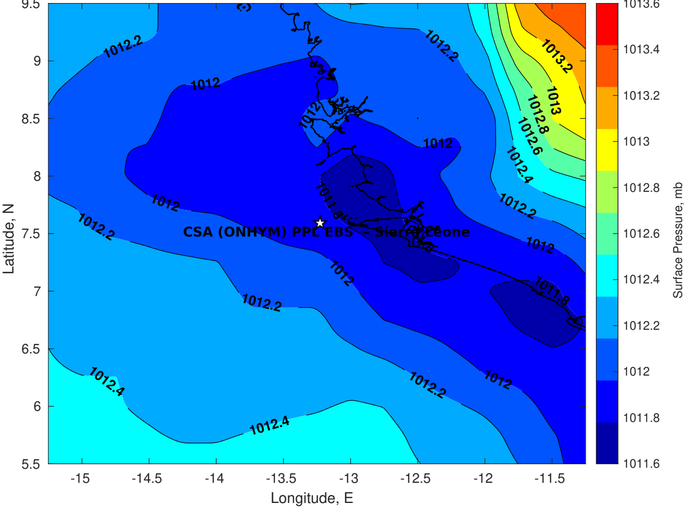
Surface Pressure (mb) for CSA (ONHYM) PPL EBS - Sierra Leone at 08-Dec-2025 00:00:00
