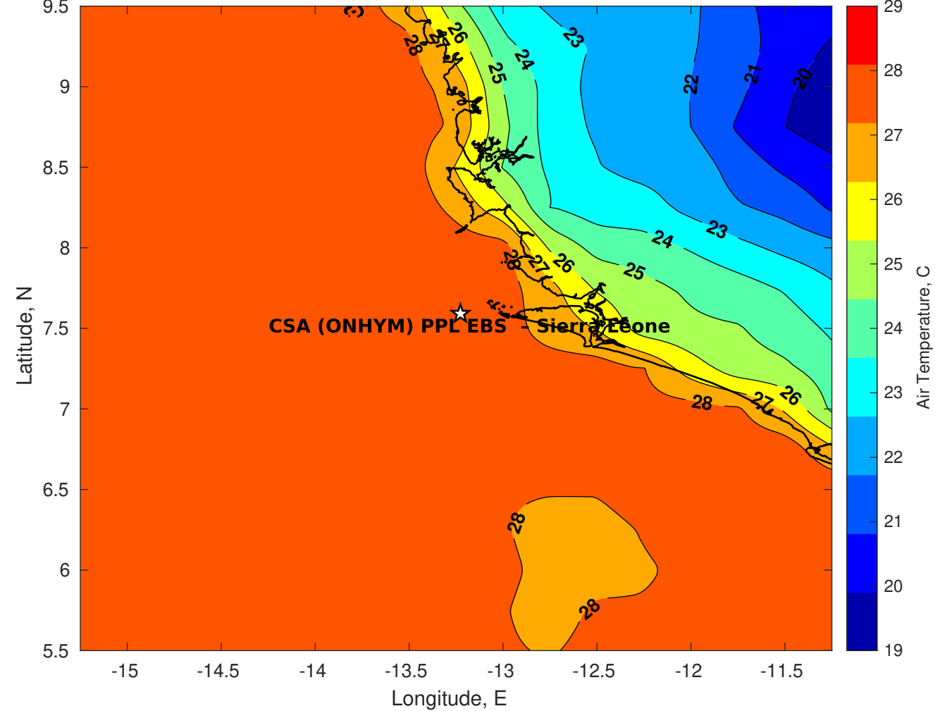
Air Temperature (C) for CSA (ONHYM) PPL EBS - Sierra Leone at 07-Dec-2025
