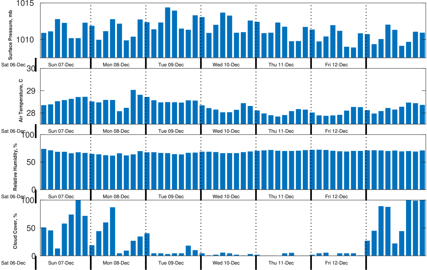
Met Forecast for CSA (ONHYM) PPL EBS - Sierra Leone from 07-Dec-2025 00:00:00 to 14-Dec-2025 00:00:00
