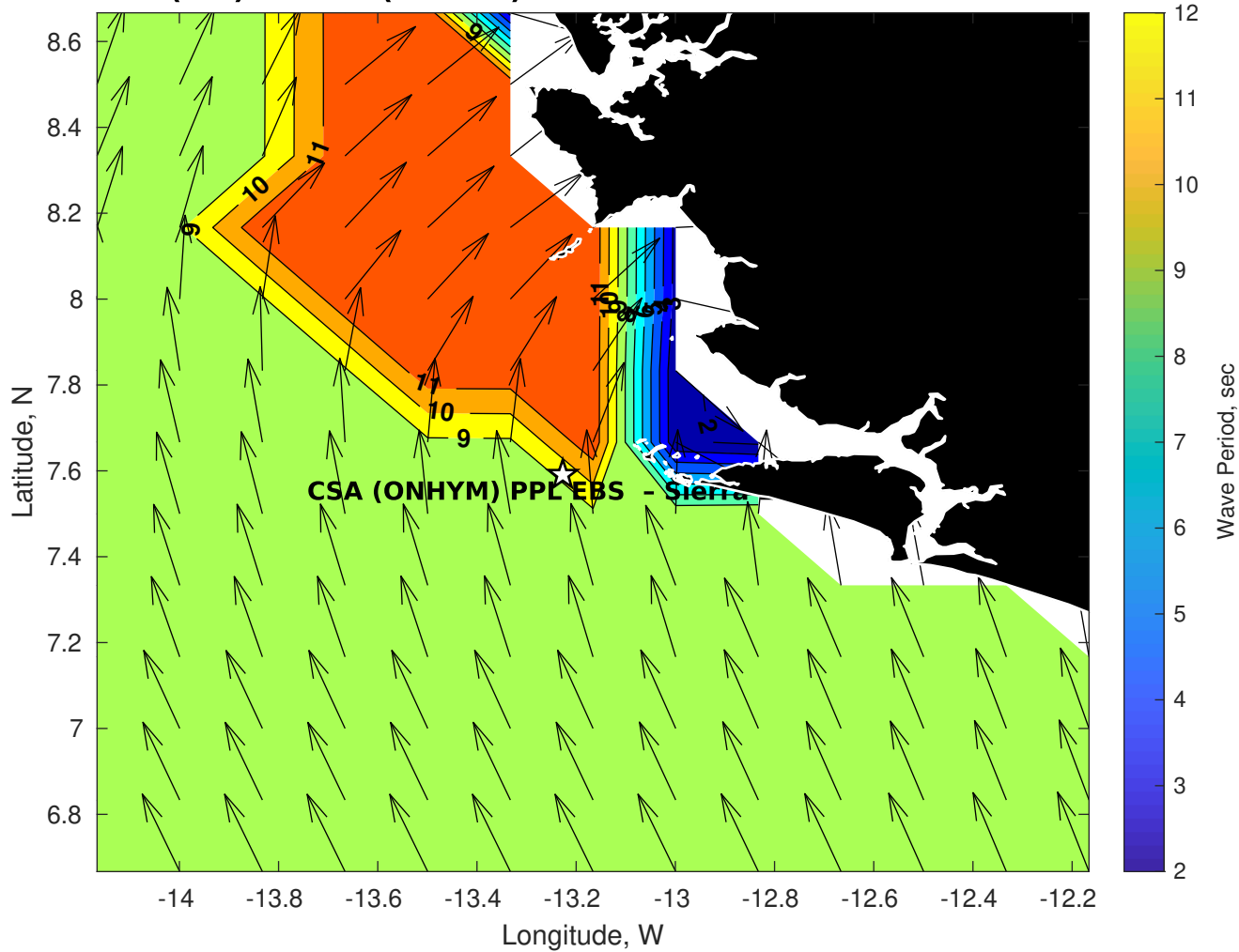
GFS Wave Period (sec) for CSA (ONHYM) PPL EBS - Sierra Leone at 07-Dec-2025 09:00:00
