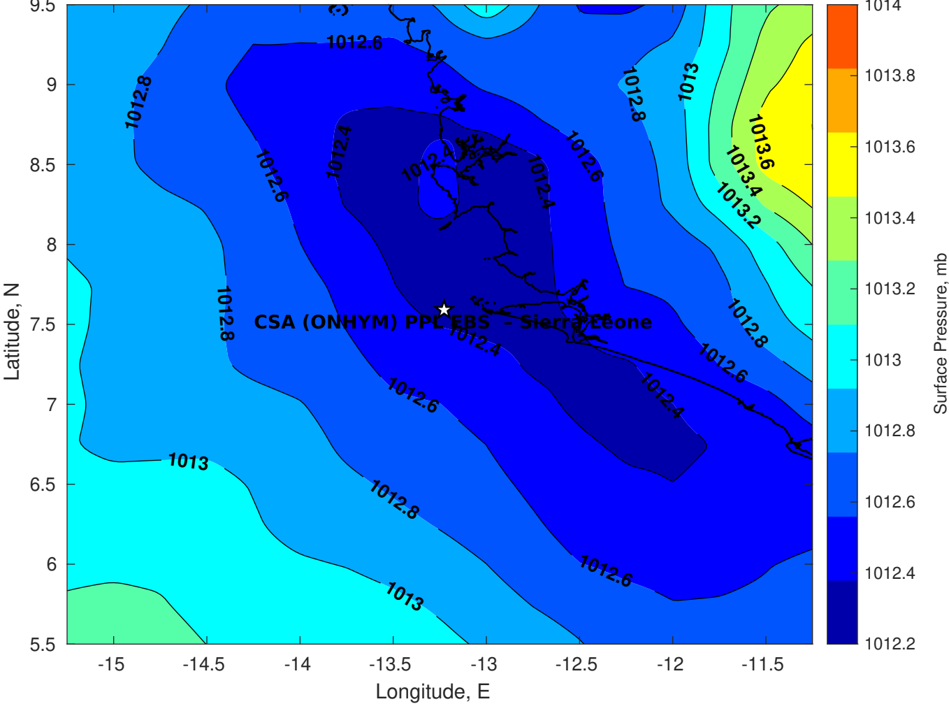
Surface Pressure (mb) for CSA (ONHYM) PPL EBS - Sierra Leone at 09-Dec-2025 00:00:00
