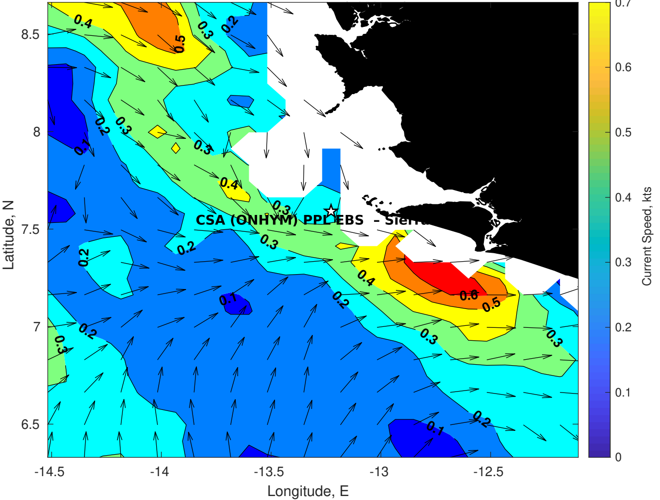
Surface Currents for CSA (ONHYM) PPL EBS - Sierra Leone at 06-Dec-2025 00:00:00
