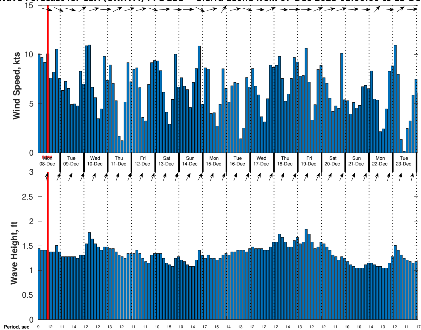
Wind & Wave Forecast for CSA (ONHYM) PPL EBS - Sierra Leone from 07-Dec-2025 01:00:00 to 23-Dec-2025 01:00:00
