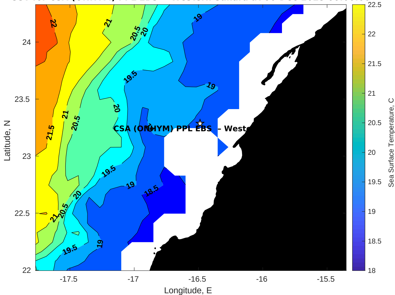
SST for CSA (ONHYM) PPL EBS - Western Sahara at 06-Dec-2025 00:00:00
