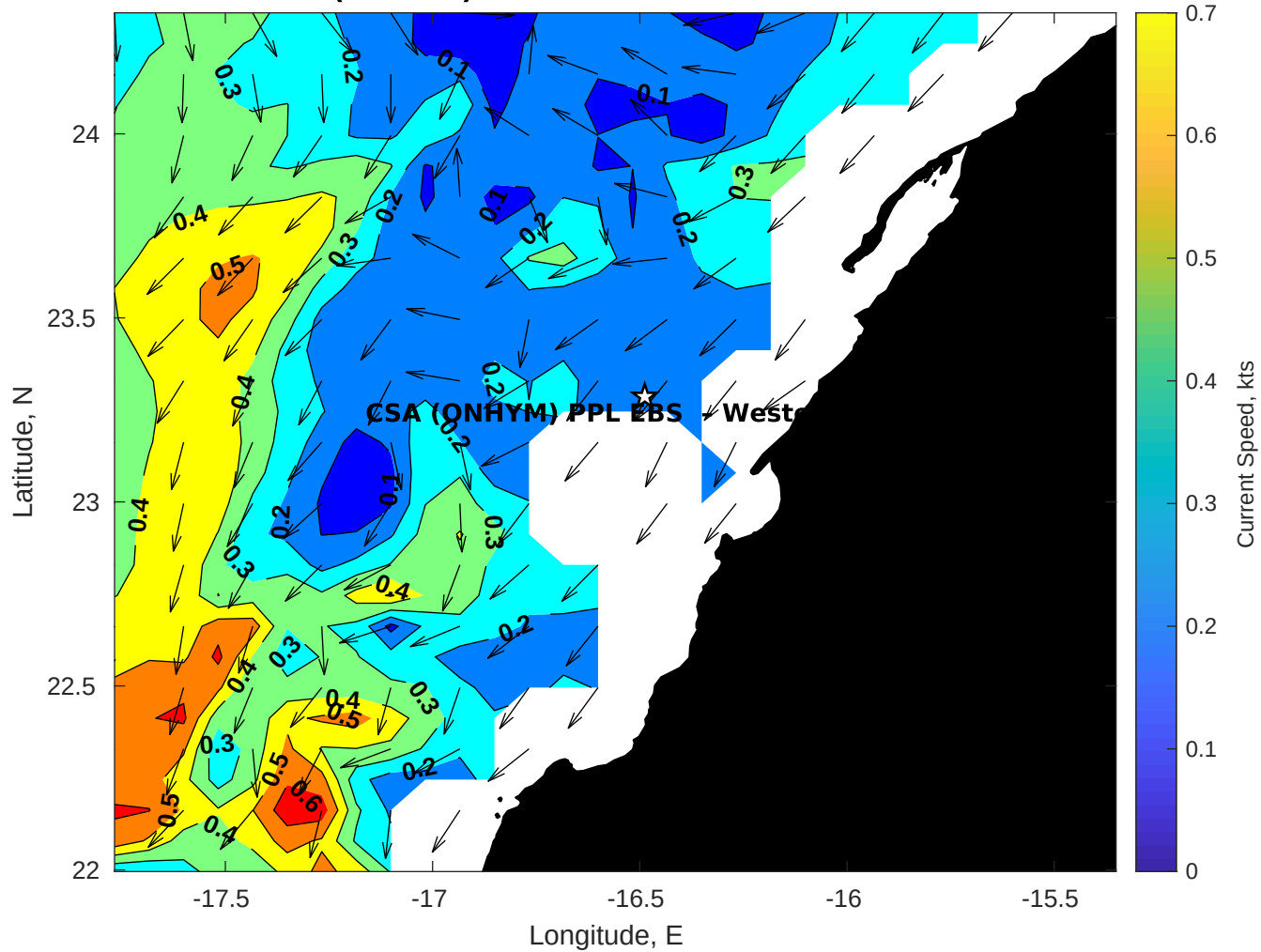
Surface Currents for CSA (ONHYM) PPL EBS - Western Sahara at 06-Dec-2025 00:00:00
