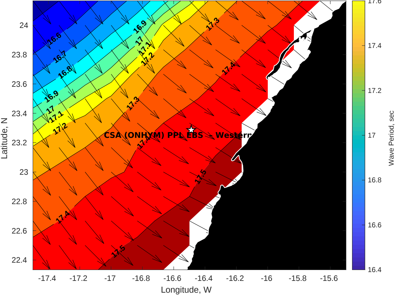
GFS Wave Period (sec) for CSA (ONHYM) PPL EBS - Western Sahara at 07-Dec-2025 09:00:00
