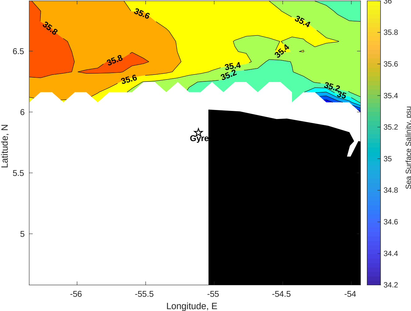
Surface Salinity for Gyre at 06-Dec-2025 00:00:00
