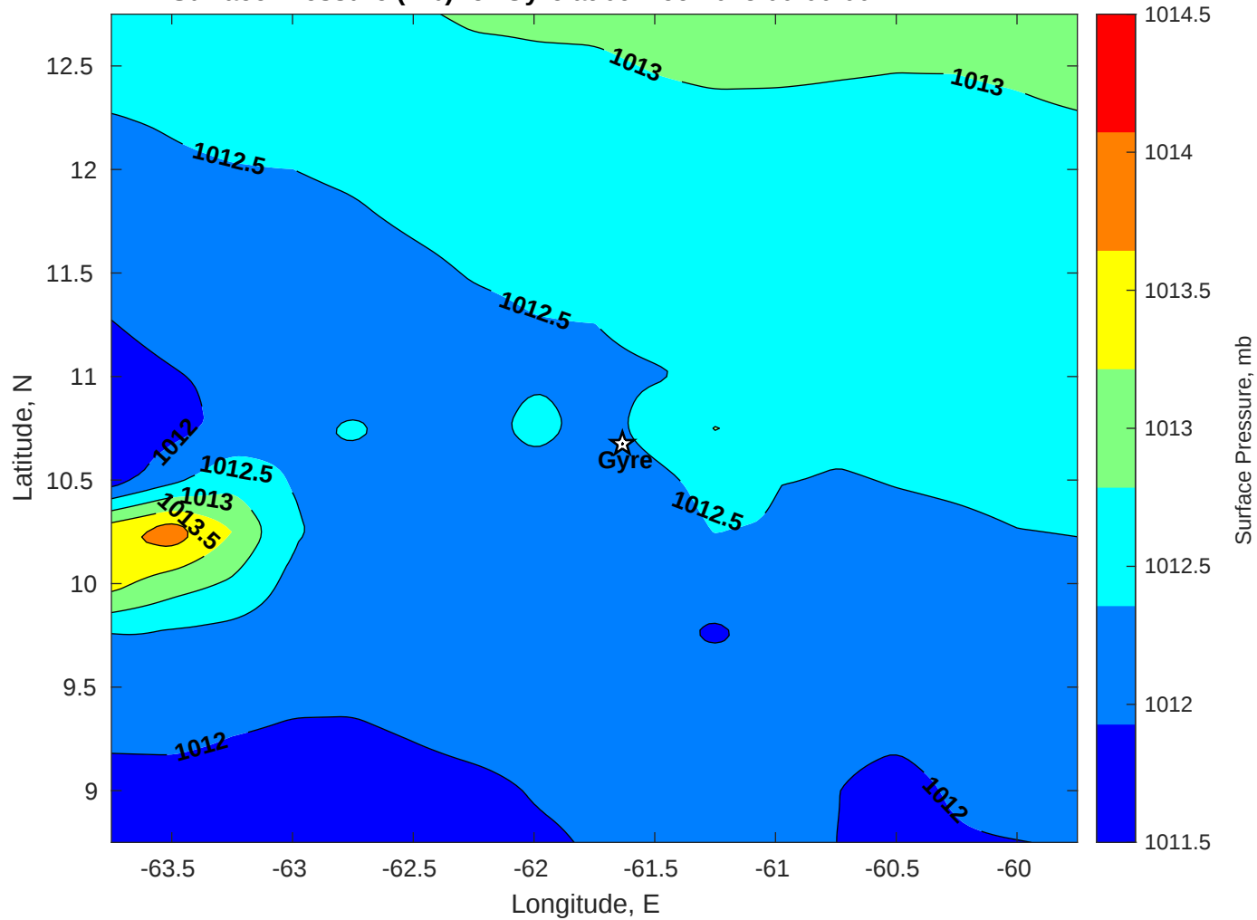
Surface Pressure (mb) for Gyre at 09-Dec-2025 00:00:00
