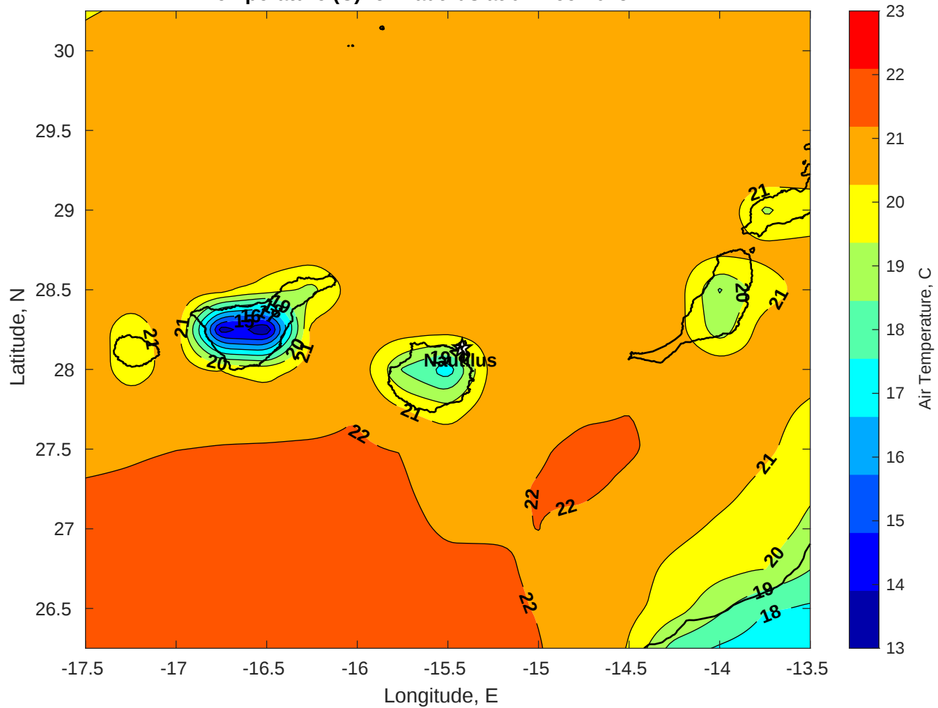
Air Temperature (C) for Nautilus at 07-Dec-2025
