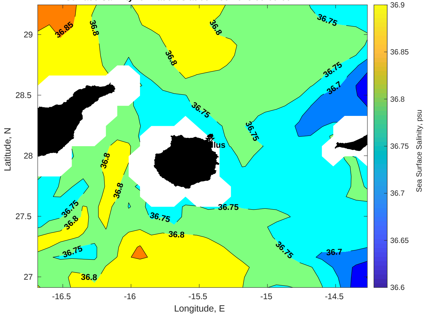
Surface Salinity for Nautilus at 06-Dec-2025 00:00:00
