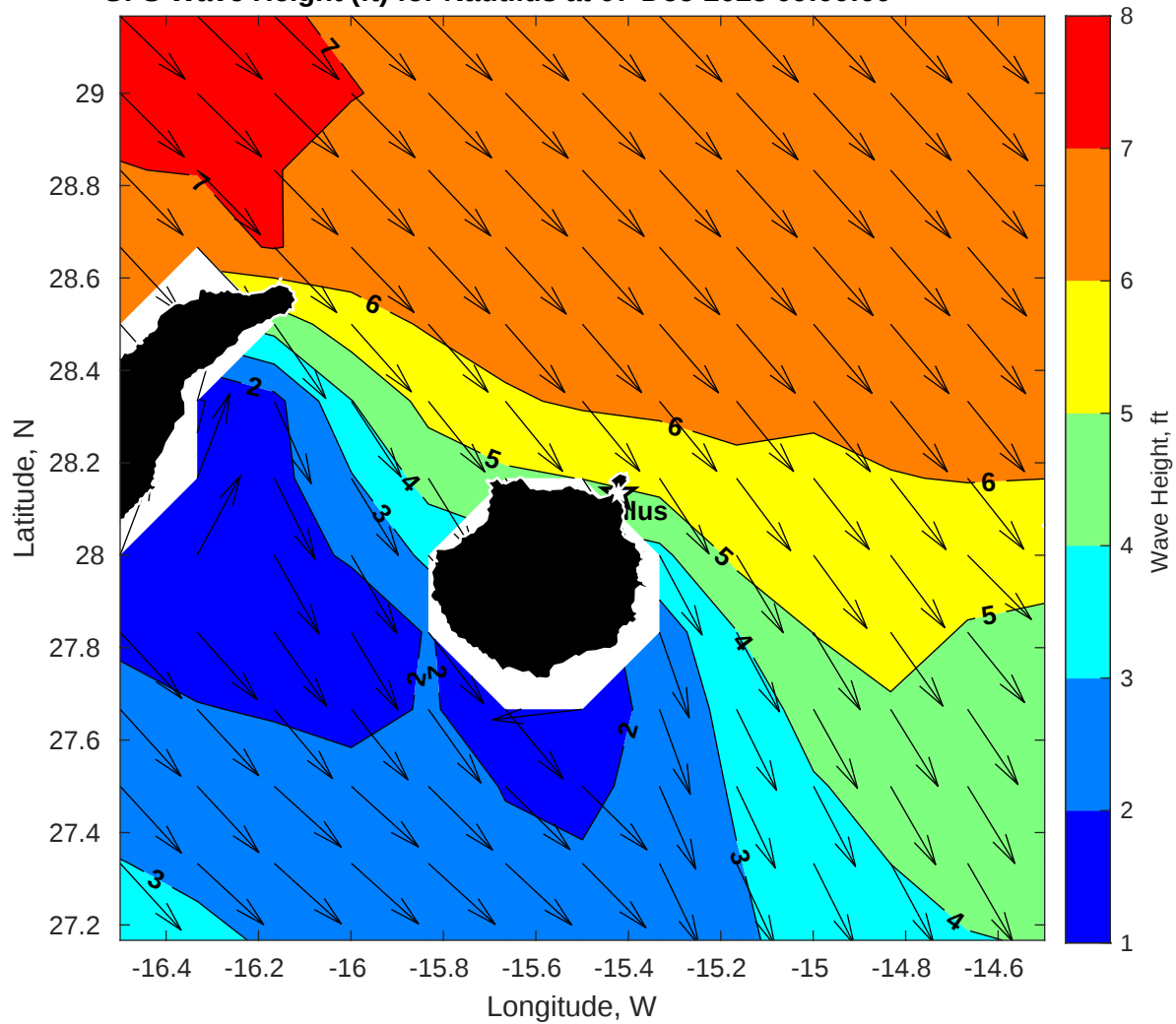
GFS Wave Height (ft) for Nautilus at 07-Dec-2025 09:00:00
