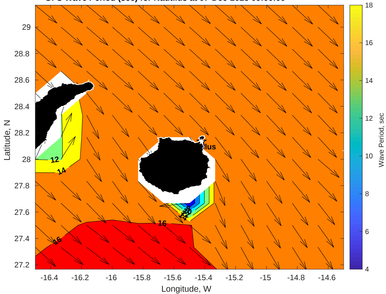
GFS Wave Period (sec) for Nautilus at 07-Dec-2025 09:00:00
