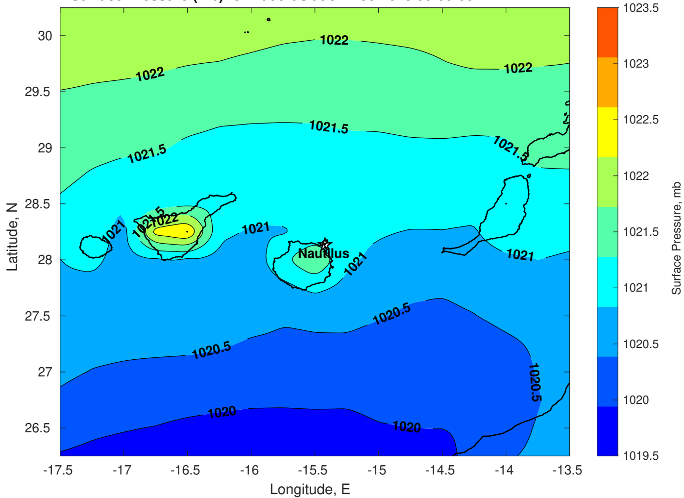
Surface Pressure (mb) for Nautilus at 07-Dec-2025 00:00:00
