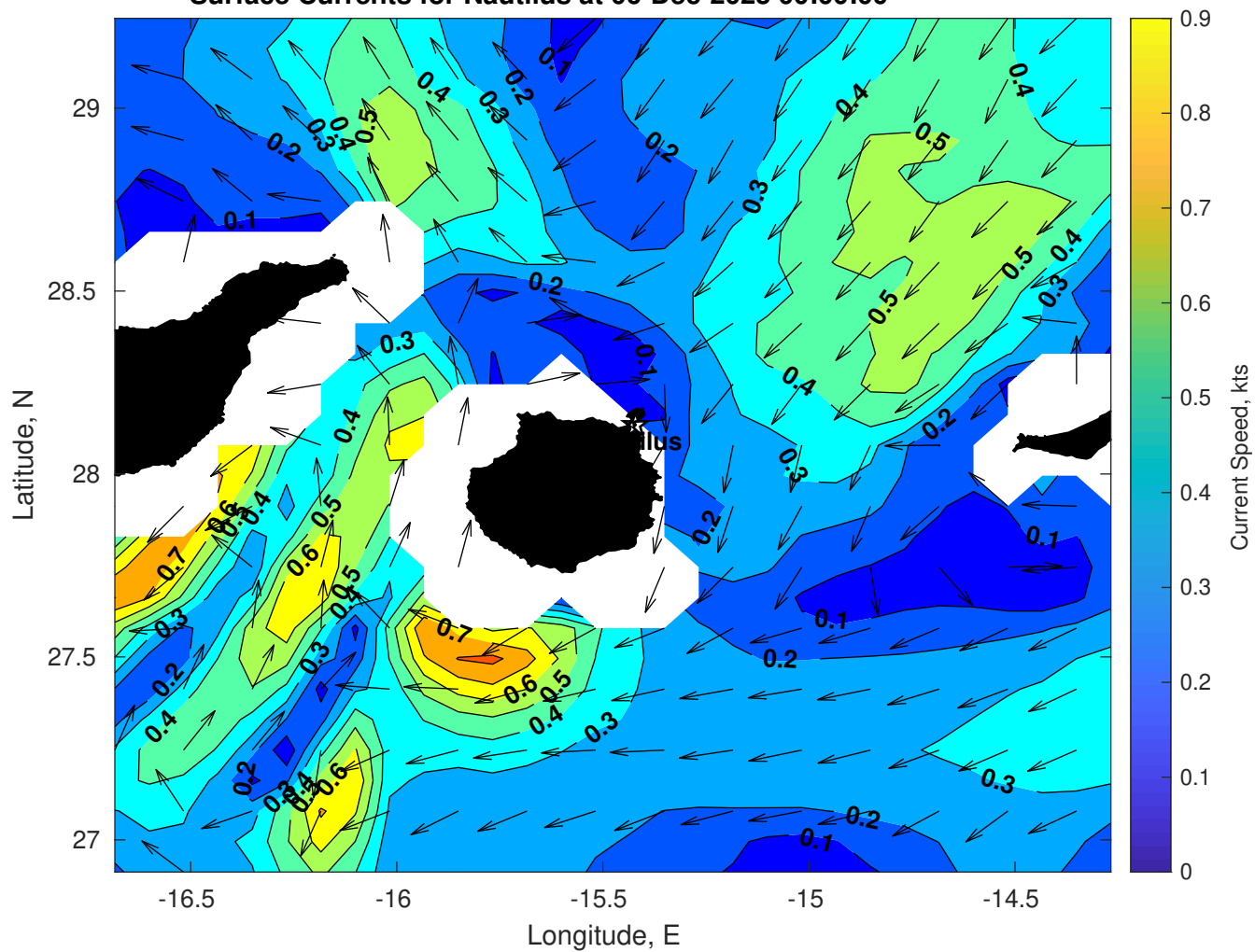
Surface Currents for Nautilus at 06-Dec-2025 00:00:00
