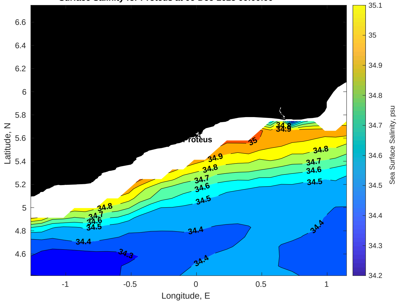
Surface Salinity for Proteus at 06-Dec-2025 00:00:00
