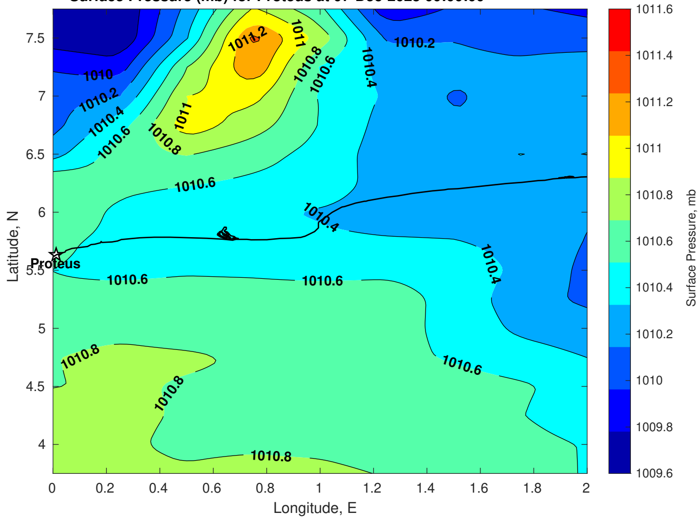
Surface Pressure (mb) for Proteus at 07-Dec-2025 00:00:00
