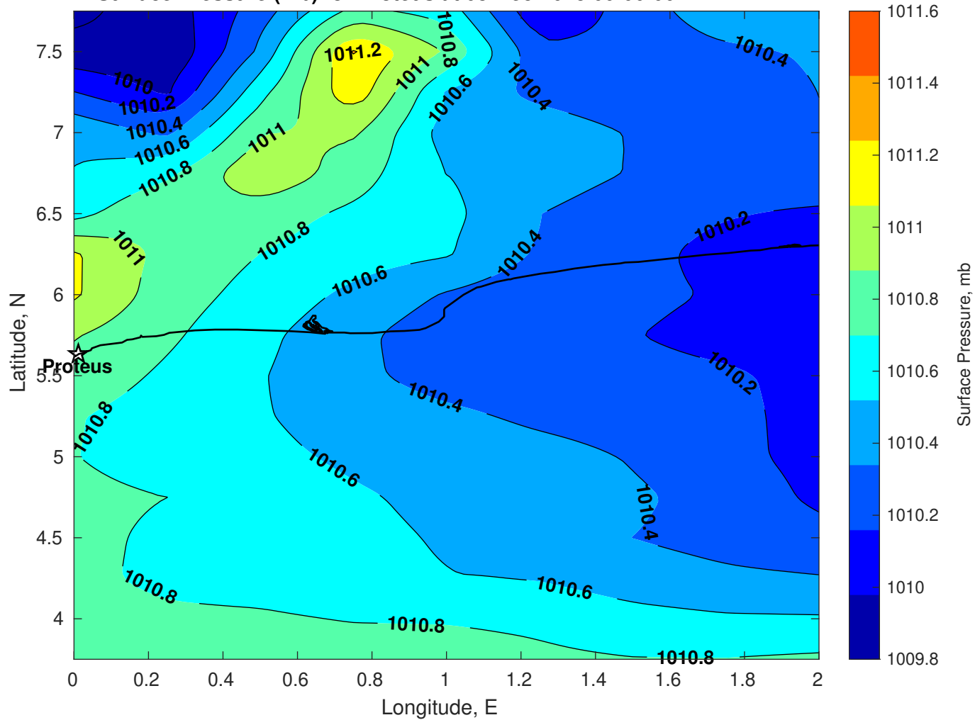
Surface Pressure (mb) for Proteus at 08-Dec-2025 00:00:00
