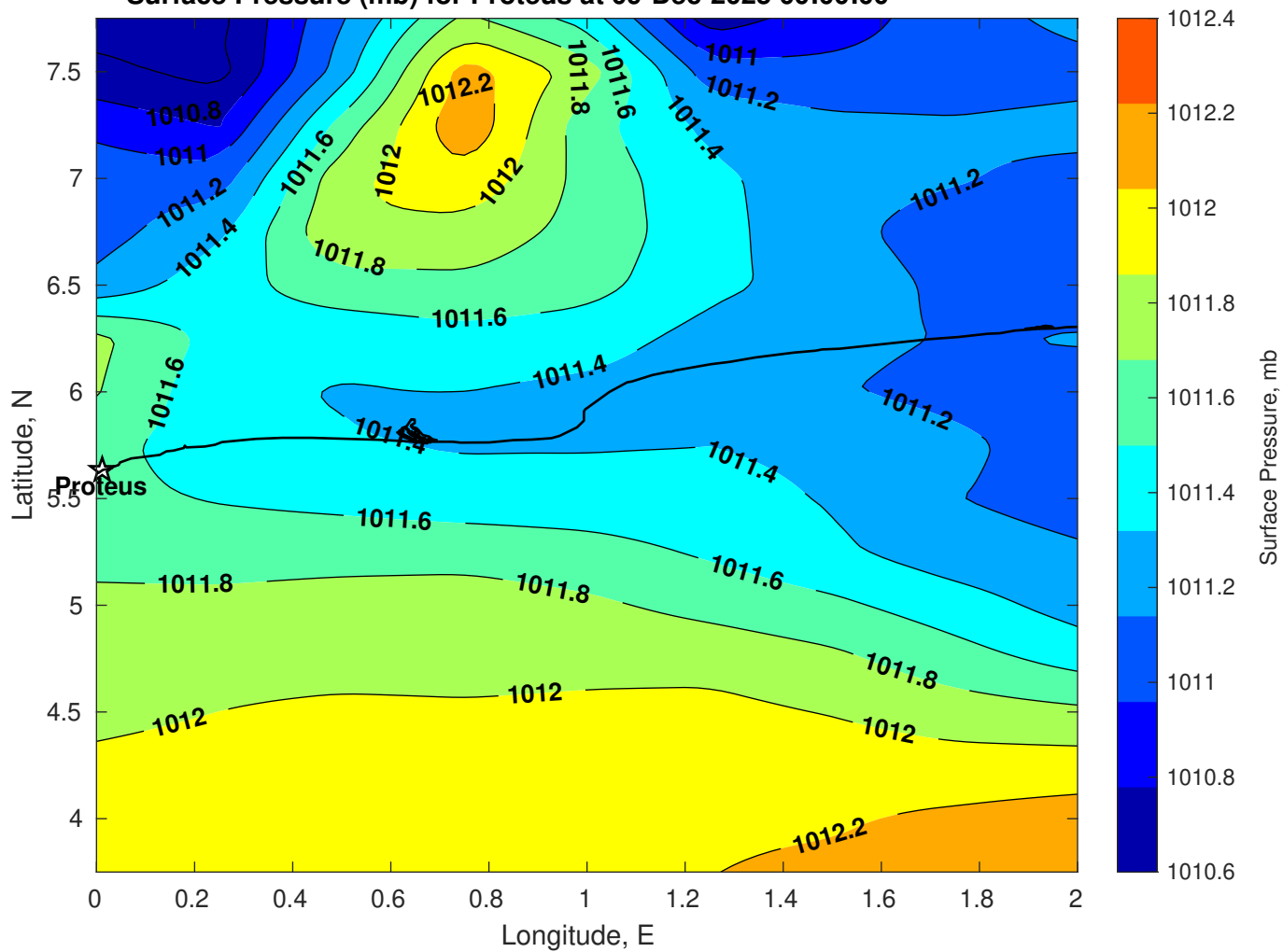
Surface Pressure (mb) for Proteus at 09-Dec-2025 00:00:00
