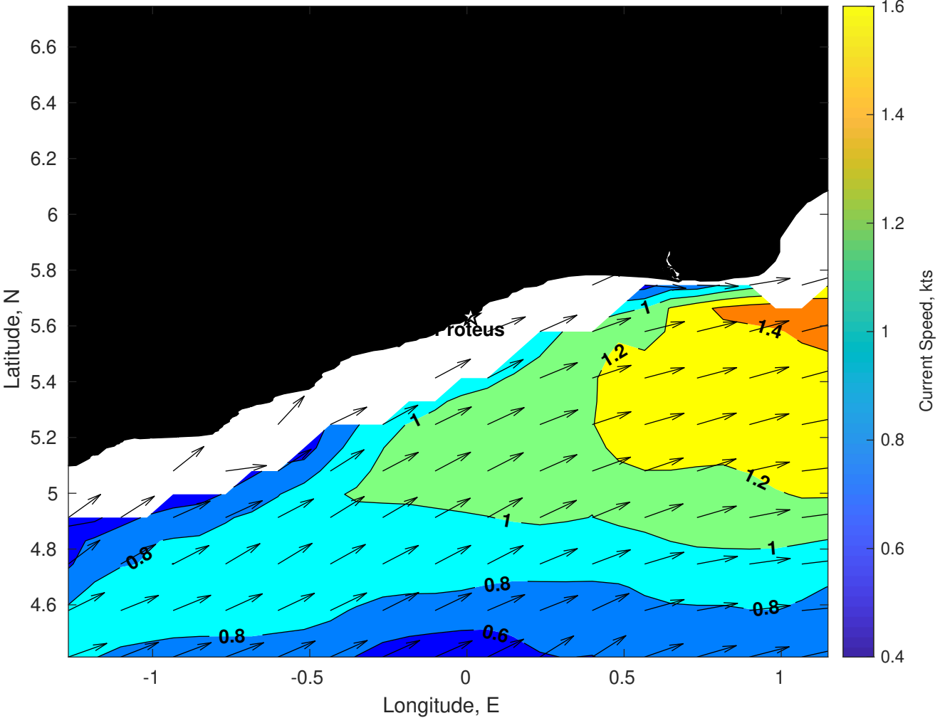
Surface Currents for Proteus at 06-Dec-2025 00:00:00
