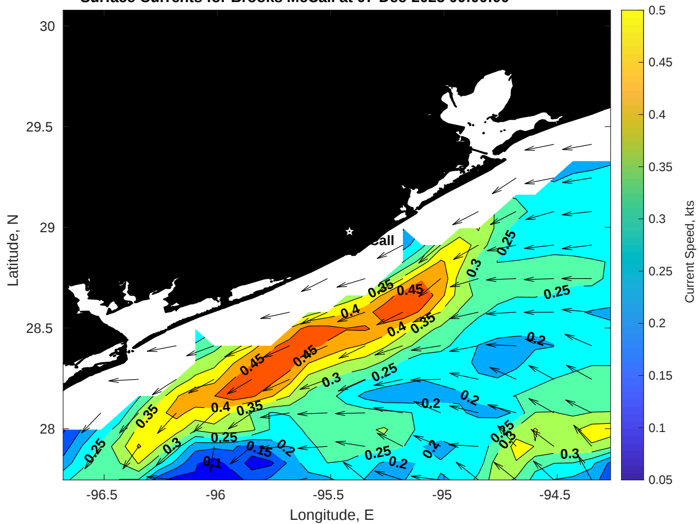
Surface Currents for Brooks McCall at 07-Dec-2025 00:00:00
