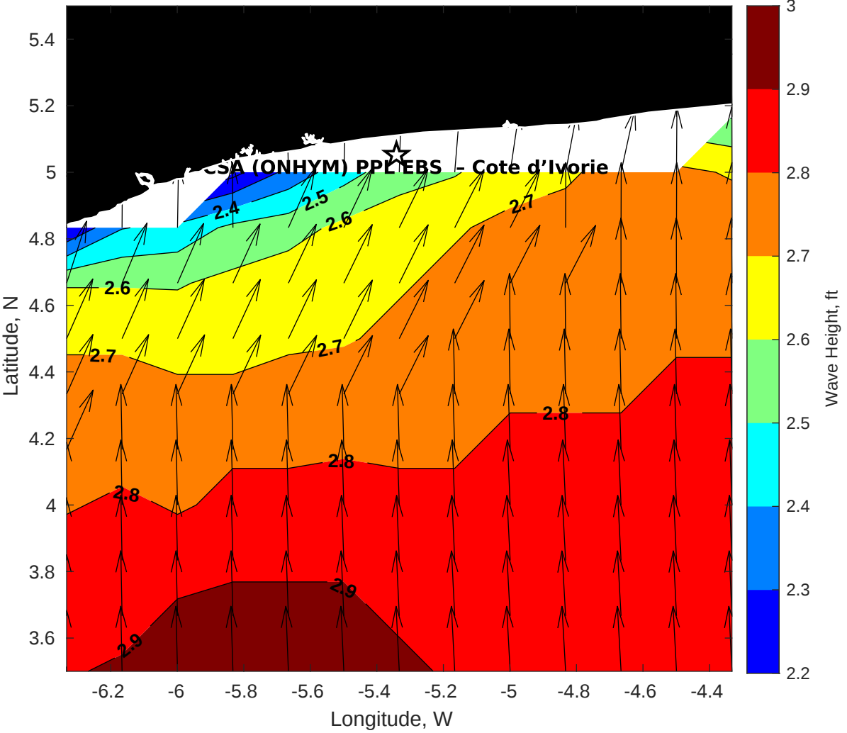
GFS Wave Height (ft) for CSA (ONHYM) PPL EBS - Cote d'Ivoire at 08-Dec-2025 09:00:00
