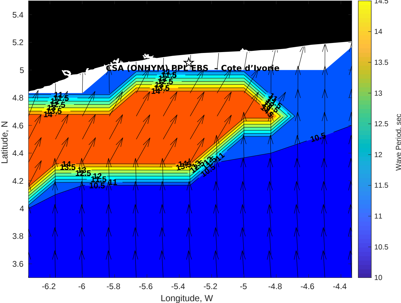
GFS Wave Period (sec) for CSA (ONHYM) PPL EBS - Cote d'Ivoire at 08-Dec-2025 09:00:00
