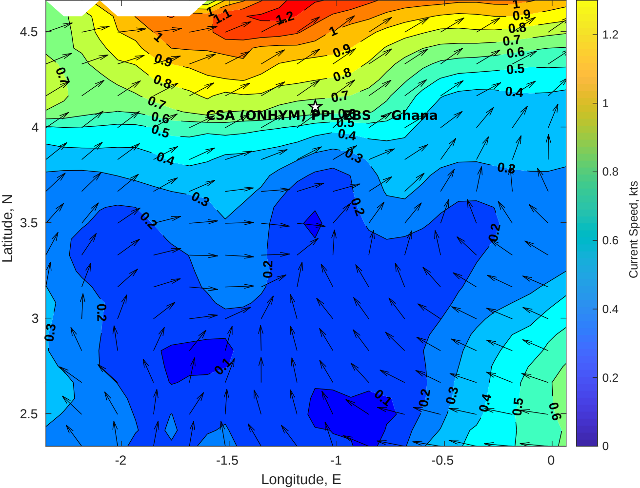
Surface Currents for CSA (ONHYM) PPL EBS - Ghana at 07-Dec-2025 00:00:00
