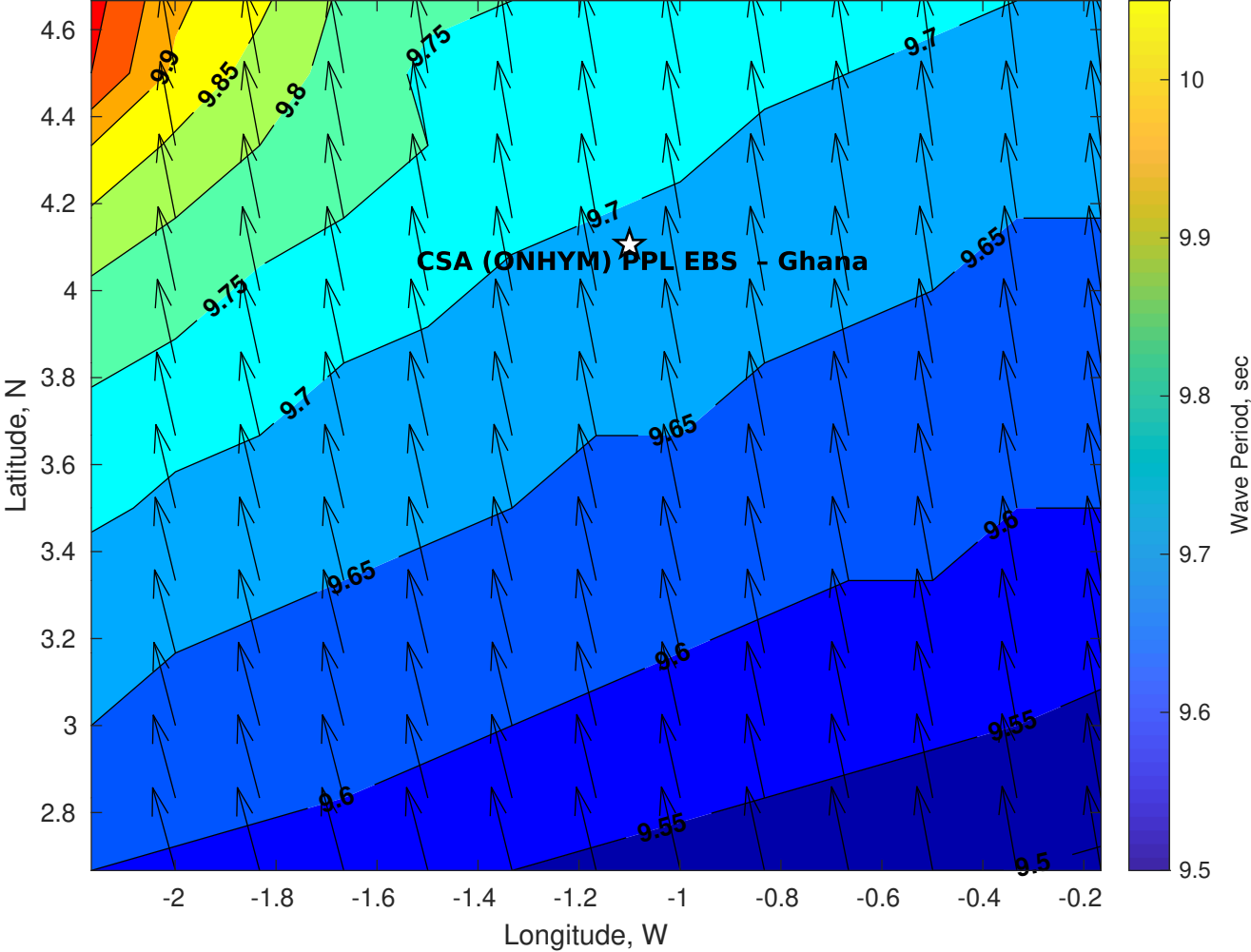
GFS Wave Period (sec) for CSA (ONHYM) PPL EBS - Ghana at 08-Dec-2025 09:00:00
