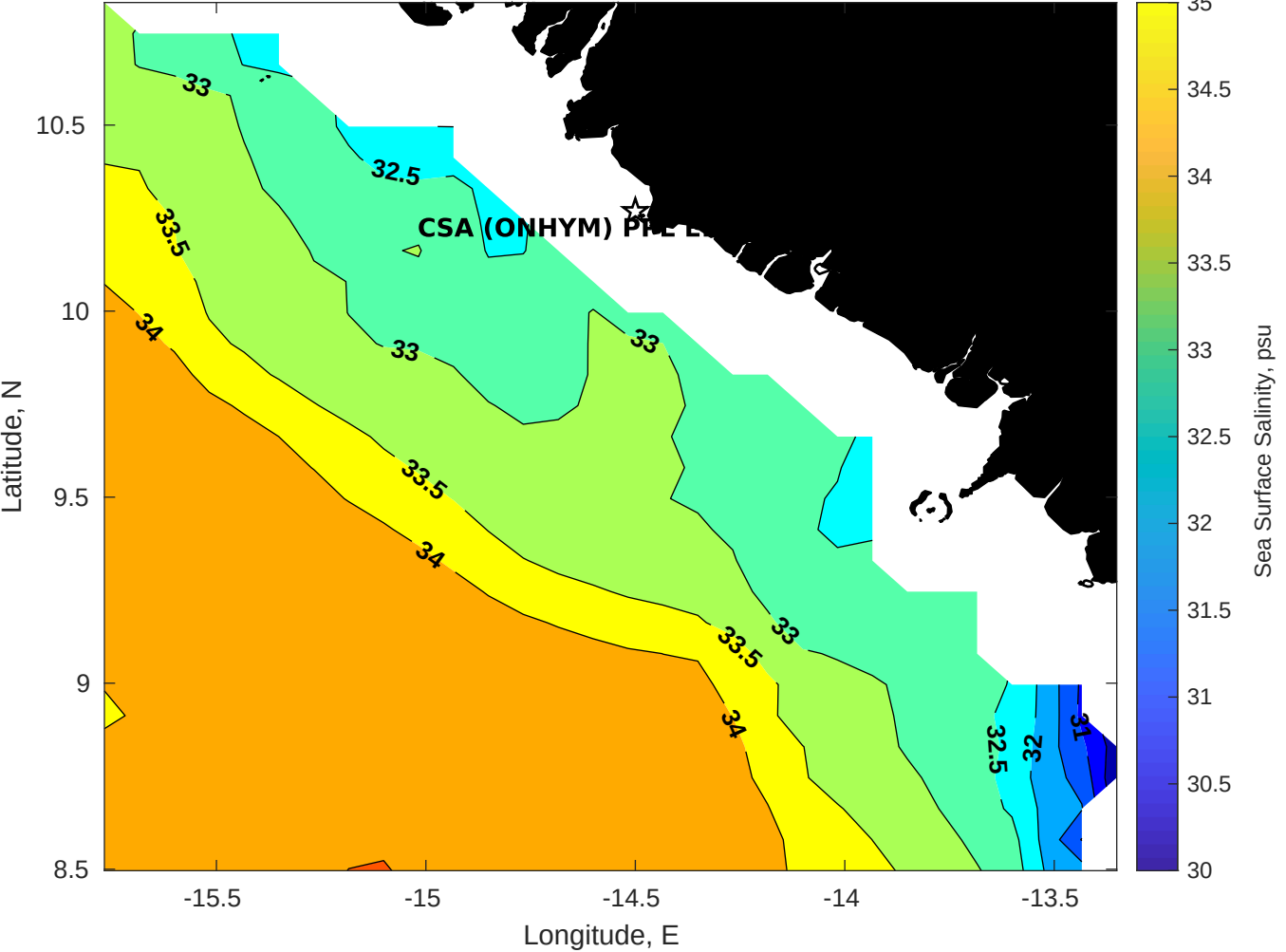
Surface Salinity for CSA (ONHYM) PPL EBS - Guinea at 07-Dec-2025 00:00:00
