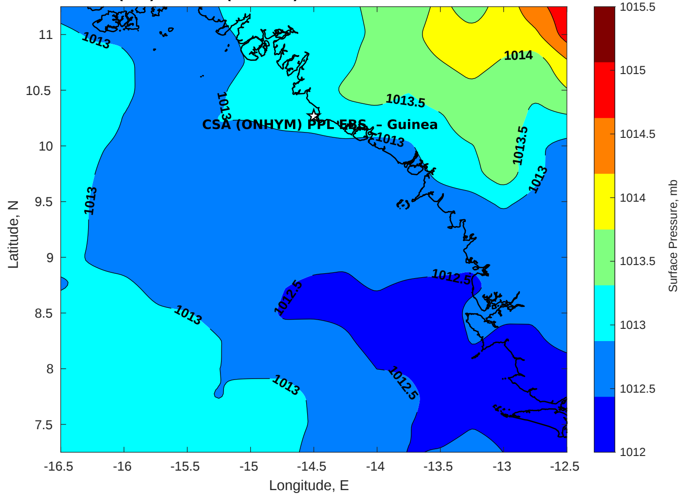
Surface Pressure (mb) for CSA (ONHYM) PPL EBS - Guinea at 10-Dec-2025 00:00:00
