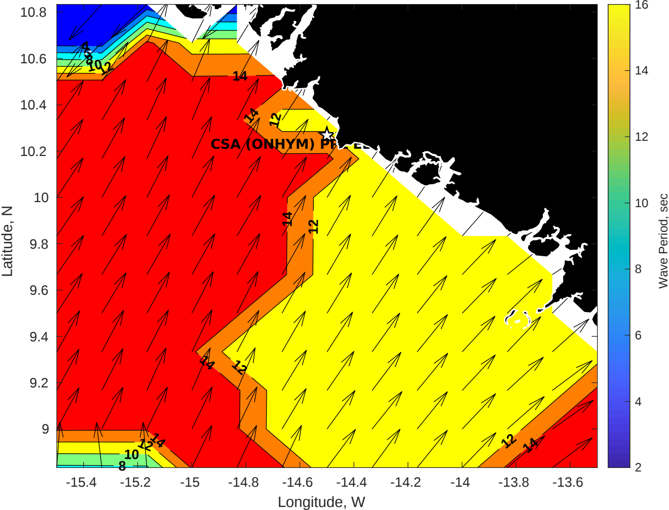
GFS Wave Period (sec) for CSA (ONHYM) PPL EBS - Guinea at 08-Dec-2025 09:00:00
