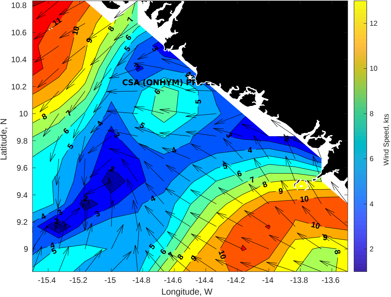
GFS Winds (kts) for CSA (ONHYM) PPL EBS - Guinea at 08-Dec-2025 09:00:00
