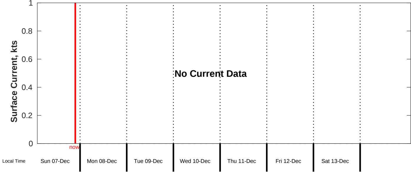
Surface Current Forecast for CSA (ONHYM) PPL EBS - Guinea from 07-Dec-2025 00:00:00 to 15-Dec-2025 00:00:00
