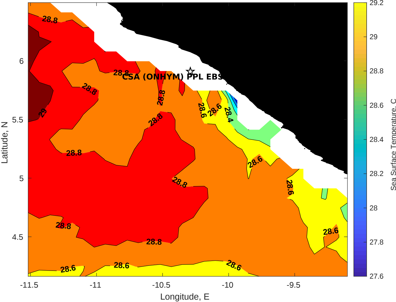
SST for CSA (ONHYM) PPL EBS - Liberia at 07-Dec-2025 00:00:00
