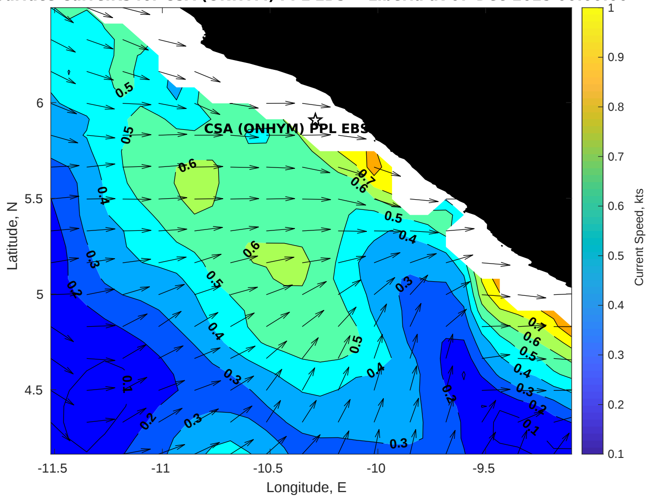
Surface Currents for CSA (ONHYM) PPL EBS - Liberia at 07-Dec-2025 00:00:00
